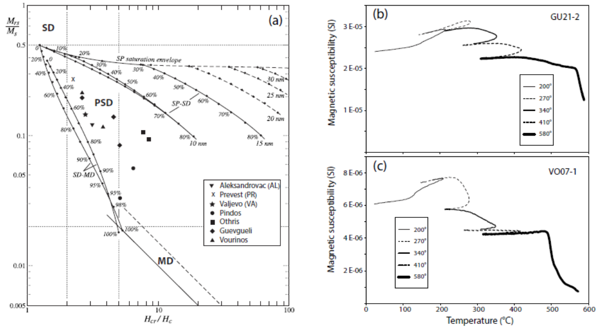
Figure 5. (a) Day plot [Day, 1977] for representative samples, showing the theoretical mixing curves for SD-MD grains (left), and SD-SP grains (right). Data fall in the PSD field of the diagram, between the SD-MD and the 10 nm SD-SP mixing curves, hence showing the occurrence of a mixed fraction containing SP, SD, MD grains. (b, c) Thermal variation of the low-field magnetic susceptibility for two representative samples from the (b) Guevgueli and (c) Vourinos ophiolite. Experiments were run under free air. Each curve consists of a combination of five heating-cooling sub-cycles, with increasing peak temperatures (shown in the enclosed rectangle) up to 580°C. Every sub-cycle consisted in heating up to a chosen peak values followed by cooling at a temperature higher than the value. Both diagrams show two blocking temperature ranges, the first at 200-410°C, and the other at ~580°C.
