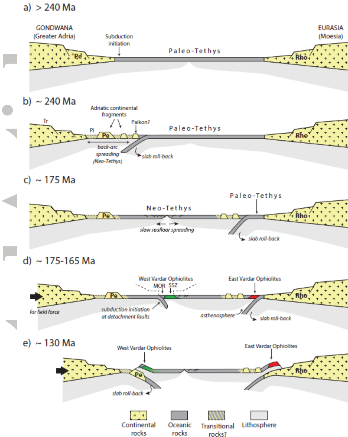
Figure 8. Speculative evolutionary cross-section of the western Tethys realm (Balkan region) from the Middle Triassic to the Early Cretaceous. (a) Before the Middle Triassic (~240 Ma) a large ocean called Paleo-Tethys existed between two regions of Pangea representing the future Eurasia and Gondwana landmasses. (b) In the Middle Triassic (~240 Ma), or perhaps even earlier in the Late Permian [Stampfli and Koruz, 2006] the Neo-Tethys Ocean started to open due to subduction initiation and Europe-ward roll-
