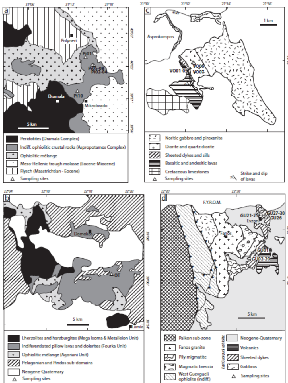
Figure 3. Simplified geological maps of the (a) Pindos, (b) Othris, (c) Vourinos, and (d) Guevgueli ophiolites, redrawn after Saccani and Photiades [2004] , Bortolotti et al. [2008] , Moore [1969] , and Saccani et al. [2008] , respectively.
