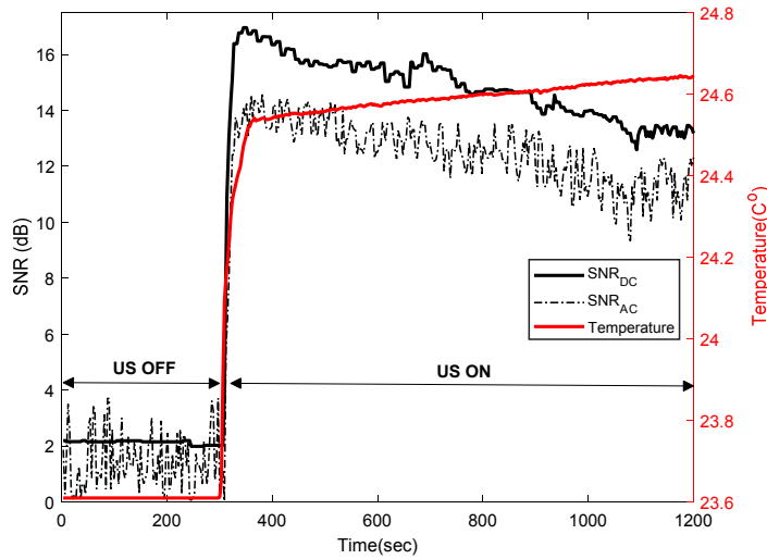
Fig. 7. UST that uses 30% duty cycle of quasi-continuous acoustic bursts to mitigate the temperature rise up to \sim 1^{\circ}\text{C} , while maintaining a significant increase in SNR for DC and AC from the CL source.
