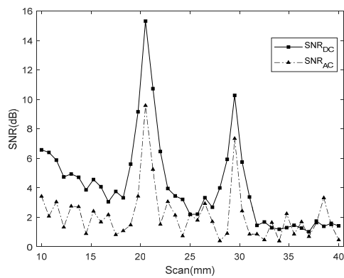
Fig. 9. SNR traces of AC and DC, where UST scans (10 to 40 mm, step size = 0.75 mm) to resolve two CL targets separated by \sim 10 mm deep inside a slab of chicken breast.
