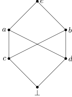
Figure 5: \mathbf{X}_\perp^\top
