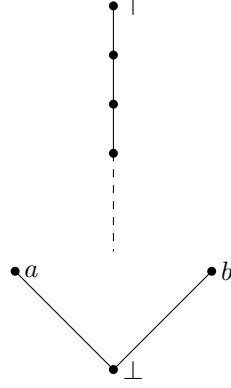
Figure 3: \mathcal{K}(\mathbb{N}^{op})_{\perp}
