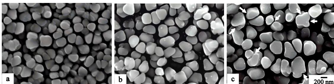
Figure 4. Morphological evolution of the secondary \gamma' precipitates after aging at 1123 K for 1 h (a), 4 h (b), and 8 h (c) in the D4 alloys. The precipitates tend towards irregular-shape morphology rather than a granular shape as the aging increased. The arrows in (c) indicates “dents” of the \gamma' particles.
