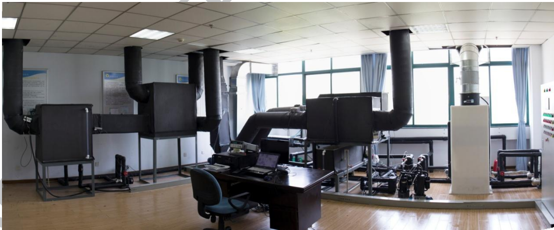
Fig. 2. Experimental setup of the hybrid vapor-compression refrigeration system.
