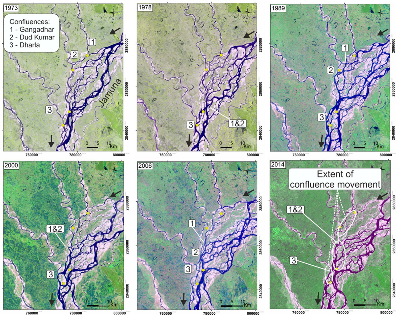
Fig. 5. Confluence of the Jamuna (Brahmaputra) River with its tributaries, from north to south: Gangadhar River (1), Dud Kumar River (2) and Dharla River (3), in the Krigram District of Northern Bangladesh. Original 1973 confluence locations marked as dark yellow points in all images. Migration of the main thalweg of the Jamuna River within its braid plain over time leads to migration and avulsion in the position of the confluences. The 2014 image is annotated with white ellipses to show the zones over which the confluences moved during the 40-year image sequence. (For interpretation of the references to colour in this figure legend, the reader is referred to the web version of this article.)
