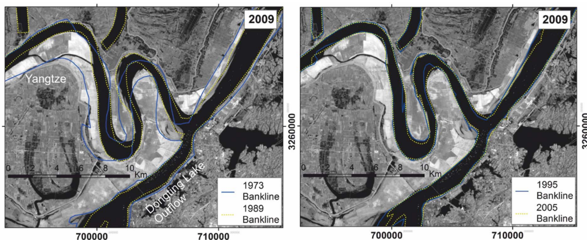
Fig. 10. Confluence of the Yangtze River and outflow from Dongting Lake, Yueyang, China. Digitised banklines from 1973, 1989, 1995 and 2005 are superimposed onto two images of the confluence planform from 2009. This sequence shows the translation and extension of meanders upstream of the pinned confluence.
