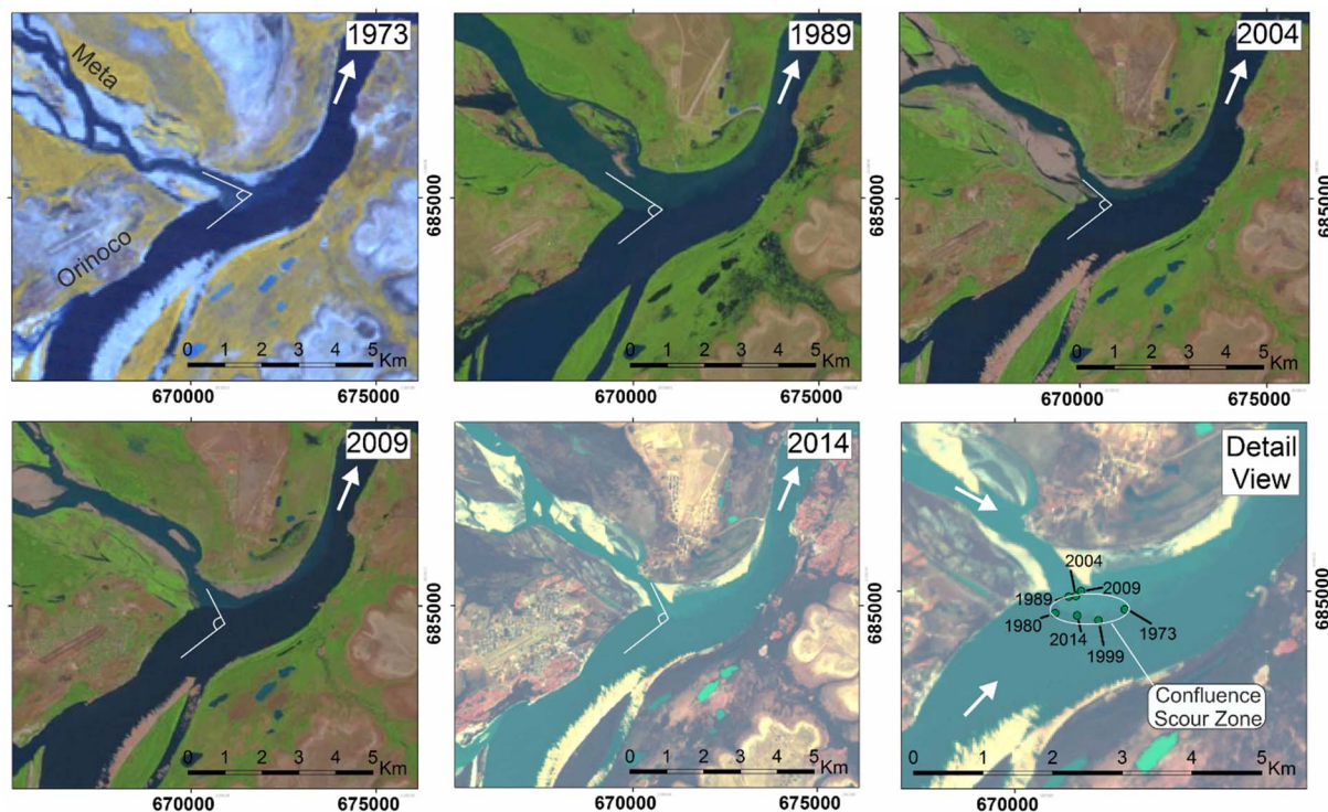
Fig. 2. Landsat image sequence showing planform changes at the junction of the River Orinoco and River Meta. The confluence position and angle shift subtly over time with formation and erosion of bars at the mouth of the Meta River. The morphological response to this bar movement is migration of the confluence within a narrow zone, shown in the detail view, approximately equal in length to the width of the Meta River channel. Note that due to paucity of cloud free images during 1973–2000, the 1989 image is at a higher river stage than the other years.
