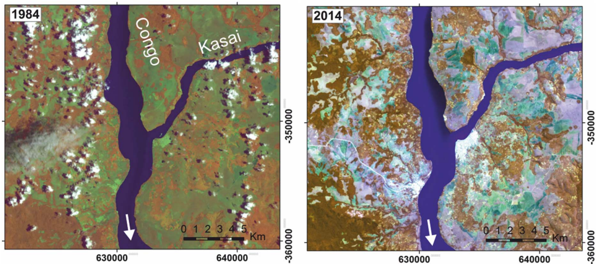
Fig. 12. Landsat images showing the confluence of the Congo and Kasai Rivers in the Democratic Republic of Congo. The rivers are heavily incised into surrounding bedrock that prevents lateral channel migration and results in a fixed confluence.
