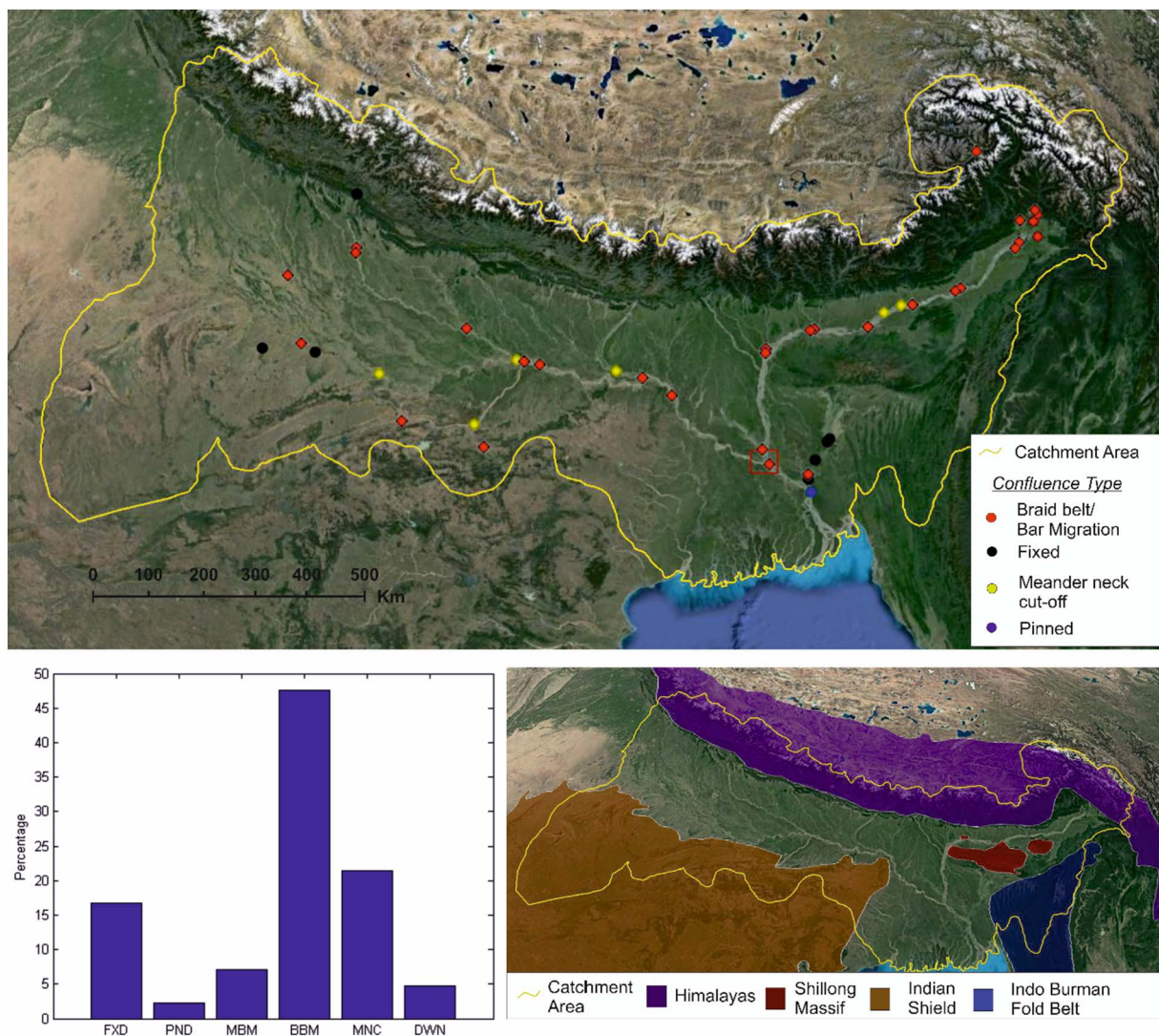
Fig. 15. Confluence classification for the Ganges-Brahmaputra-Meghna basin ( n = 42 ). Insets show the percentage occurrence of confluence types in the basin (FXD — Fixed, PND — Pinned, MBM — Mouth Bar Migration, BBM — Braid Belt Migration, MNC — Meander Neck Cut-off, DWN — Downstream Migration), and the broad geological zones in the basin, the non-highlighted areas in the geological map being lowland sedimentary basin. The majority of confluences ( n = 23 ) are mobile through braid bar/belt migration due to high sediment loads from Himalayas.
