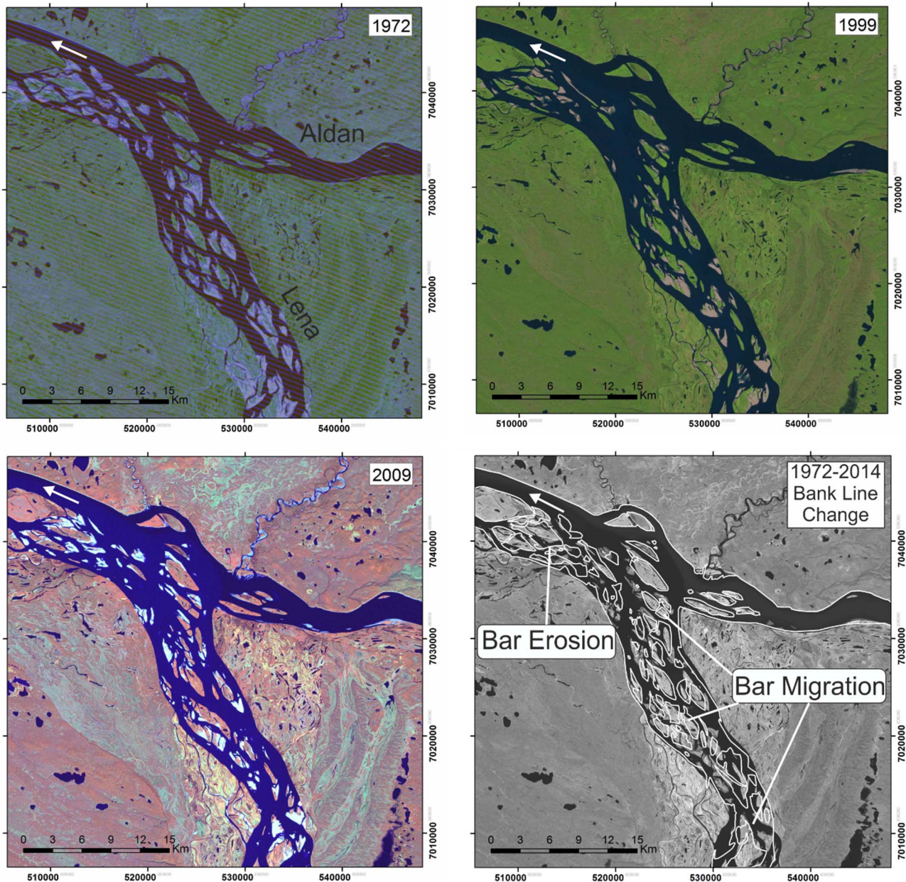
Fig. 3. Landsat images showing planform change at the confluence of Lena and Aldan rivers, Siberia, Russia from 1972 to 2014. Erosion at bar heads leads to very slow downstream migration of bars into the confluence zone; there is also gradual bar/bank erosion in the zone downstream of the confluence.
