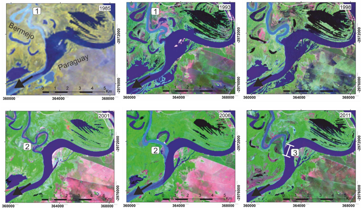
Fig. 6. Landsat images from 1985 to 2011 showing confluence morphodynamics of the Paraguay and Bermejo Rivers, Argentina. Between 1985 and 1993 a meander cut-off (1) upstream in the Bermejo River, coupled with meander loop extension in the vicinity of the confluence, causes an increase in confluence angle and downstream migration. A second cut-off between 2001 and 2006 (2) leads to an upstream shift in confluence location and a decrease in confluence angle. The maximum extent of confluence location change, just over 1 km, is illustrated by label 3, and is equivalent to approximately one post-confluence channel width.
