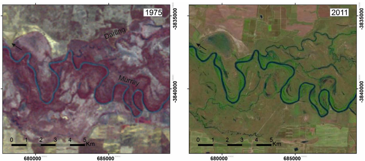
Fig. 13. Landsat images showing the confluence of the Murray and Darling rivers in Australia. The images show abandoned meander loops in the floodplain surface suggesting historic channel mobility, but over the 36-year image sequence there is no evidence of active meandering and the confluence position remains fixed.
