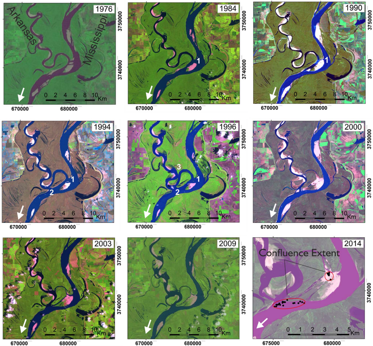
Fig. 7. Landsat images showing the confluence of the Mississippi and Arkansas rivers, USA. Downvalley migration of meander bends in the Arkansas River, coupled with extension and cut-off of individual bends, leads to rapid, avulsive switching of the confluence location on annual timescales. The point bar labelled (1) becomes attached and detached, thus shifting confluence location by \sim 3 km between 1976 and 1992. In 1994, the gradual downvalley migration of meander bends in the preceding years leads to a neck cut-off (2) and shift of confluence location. A further cut-off upstream in the Arkansas River (3) promotes abandonment of the original channel and rapid infilling. The 2014 image shows confluence locations for every year from 1976 to 2014 for which an image is available, and highlights the spatial extent of confluence influence over this period.
