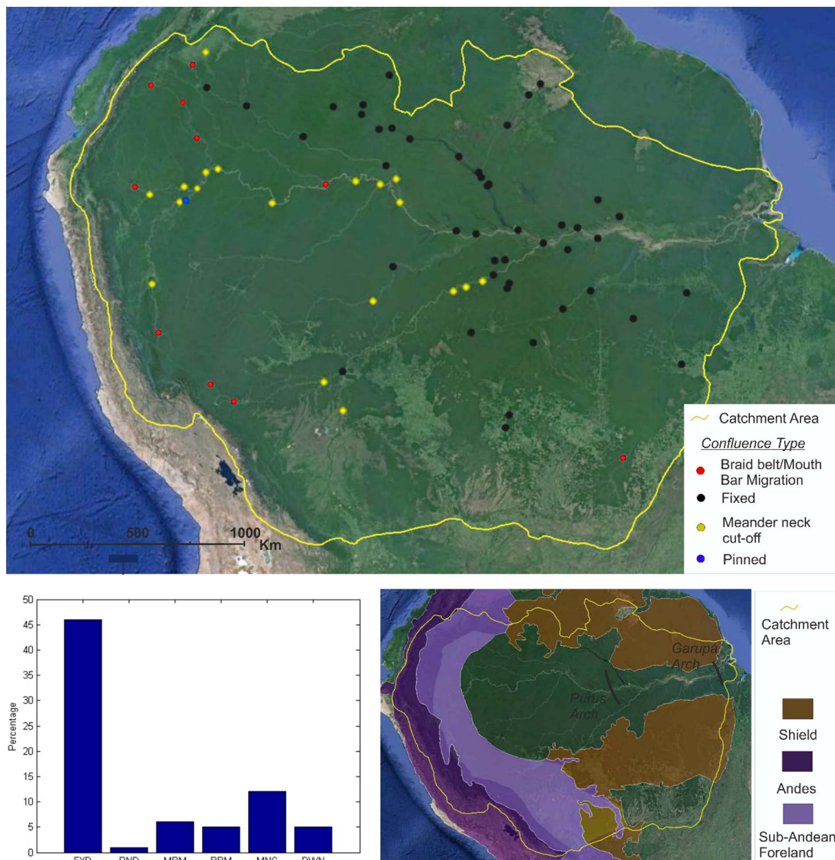
Fig. 16. Confluence classification for the Amazon basin ( n = 75 ). Insets show the percentage occurrence of confluence types in the basin (FXD — Fixed, PND — Pinned, MBM — Mouth Bar Migration, BBM — Braid Belt Migration, MNC — Meander Neck Cut-off, DWN — Downstream Migration), and the broad geological zones in the basin, the non-highlighted areas in the geological map are lowland sedimentary basin. The majority of confluences are fixed ( n = 46 ), with mobile confluences of meander neck cut-off type in the upper trough and sub-Andean foreland and braid bar/belt migratory type in Andes.
