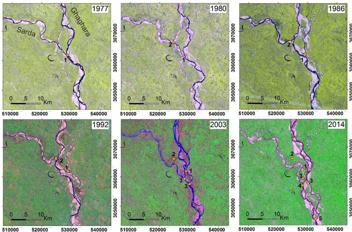
Fig. 8. Landsat images showing confluence of the Ghaghara River (flowing north to south) and Sarda River (flowing broadly west-east), Uttar Pradesh, India. Migration and avulsion of the lower Ghaghara channel drives the movement of the confluence location from (1) in 1977 to (2) in 1986 where a dual junction is present, to (3) in 2003 and finally two separate confluences (4 & 5) around 12 km apart in 2014. The 2014 image shows the extent of confluence movement is 23 km from (2) to (5). Note that confluence location also migrates approximately 1 km during the intra-avulsion periods (1) between 1977 and 1980 and (2) between 1986 and 1992.
