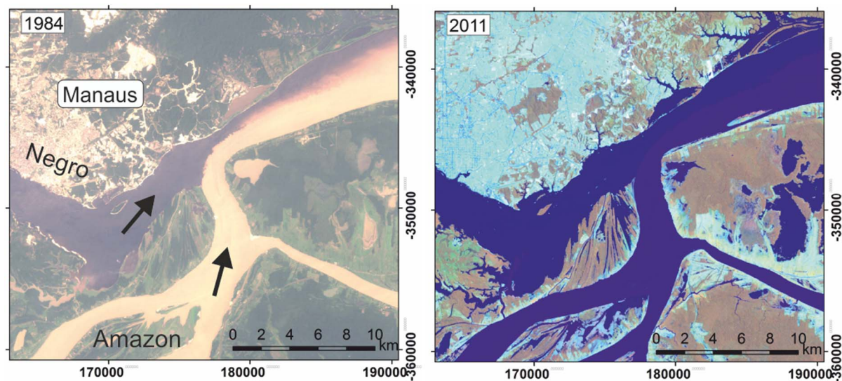
Fig. 11. Confluence of the Solimões and Negro rivers, Brazil. Despite evidence of accretional features in the floodplain associated with channel migration, and slight movement of the entrance point of the Solimões River into the junction, the confluence has remained essentially fixed over decadal timescales. Note growth of city of Manaus (light blue) in the 2011 false colour image with associated bank development/reinforcement. (For interpretation of the references to colour in this figure legend, the reader is referred to the web version of this article.)
