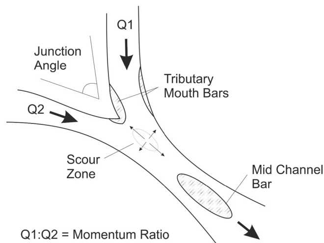
Fig. 1. Cartoon showing the major morphological features of a channel confluence as referred to in the text.
