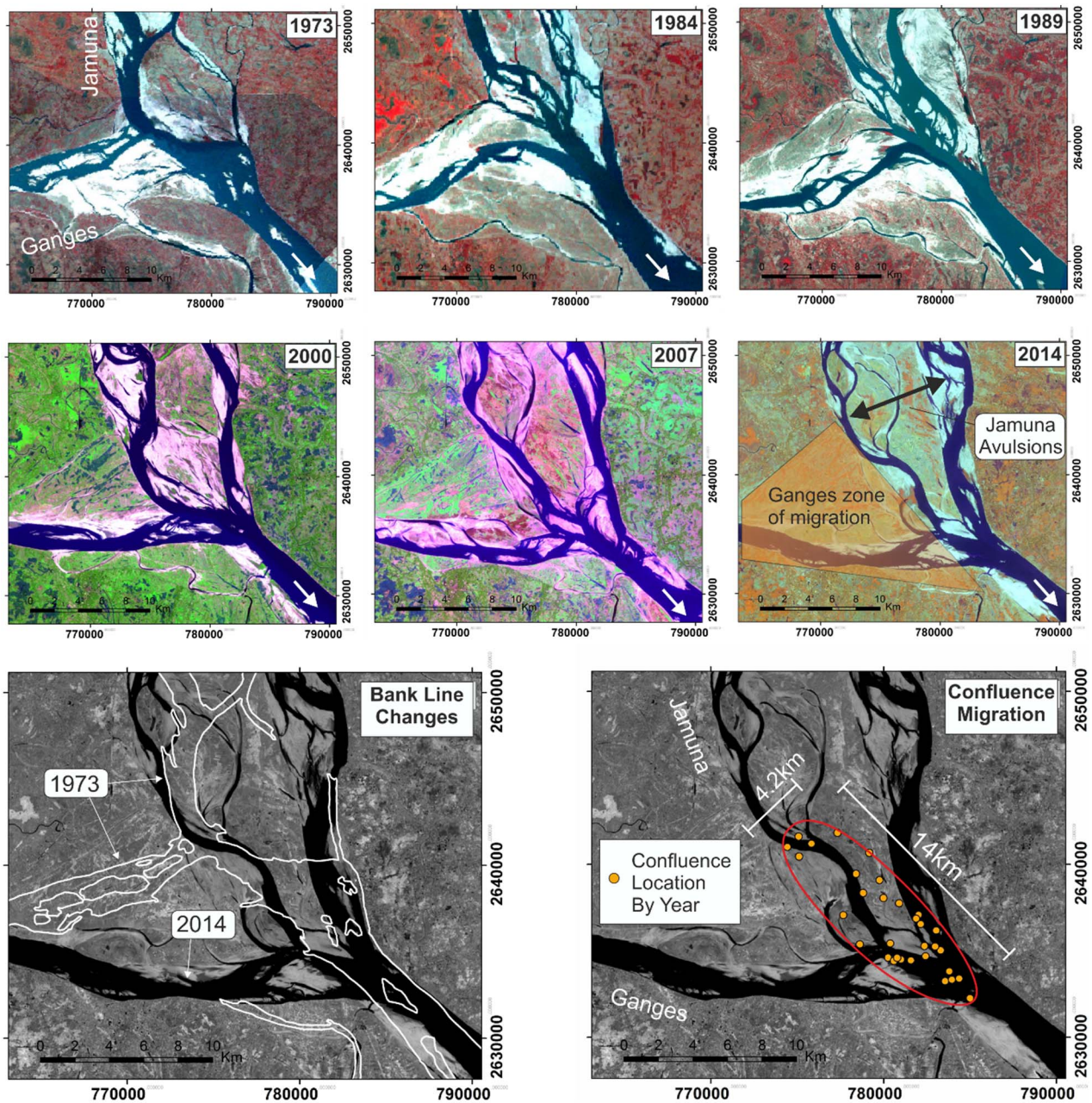
Fig. 4. Sequence of six Landsat images of the junction of the Ganges and Jamuna rivers, Bangladesh, over the period 1973–2014, with additional panels comparing banklines between 1973 and 2014 and the overall confluence migration by year. The Ganges River has migrated in a southerly direction over the image sequence, which appears to be part of a cyclical north-south migration of this channel downstream of a nodal point (see text); a proposed zone for this migration is shown on the 2014 panel. In addition, periodic changes in orientation and position of dominant flow in the Jamuna River are evident, with the extent of this variation being indicated by the black arrow on the 2014 panel. The combined result of these two modes of tributary movement at the junction results in extensive changes in confluence position over time, which over 40 years encompasses a zone 14 km long and 4.2 km wide.
