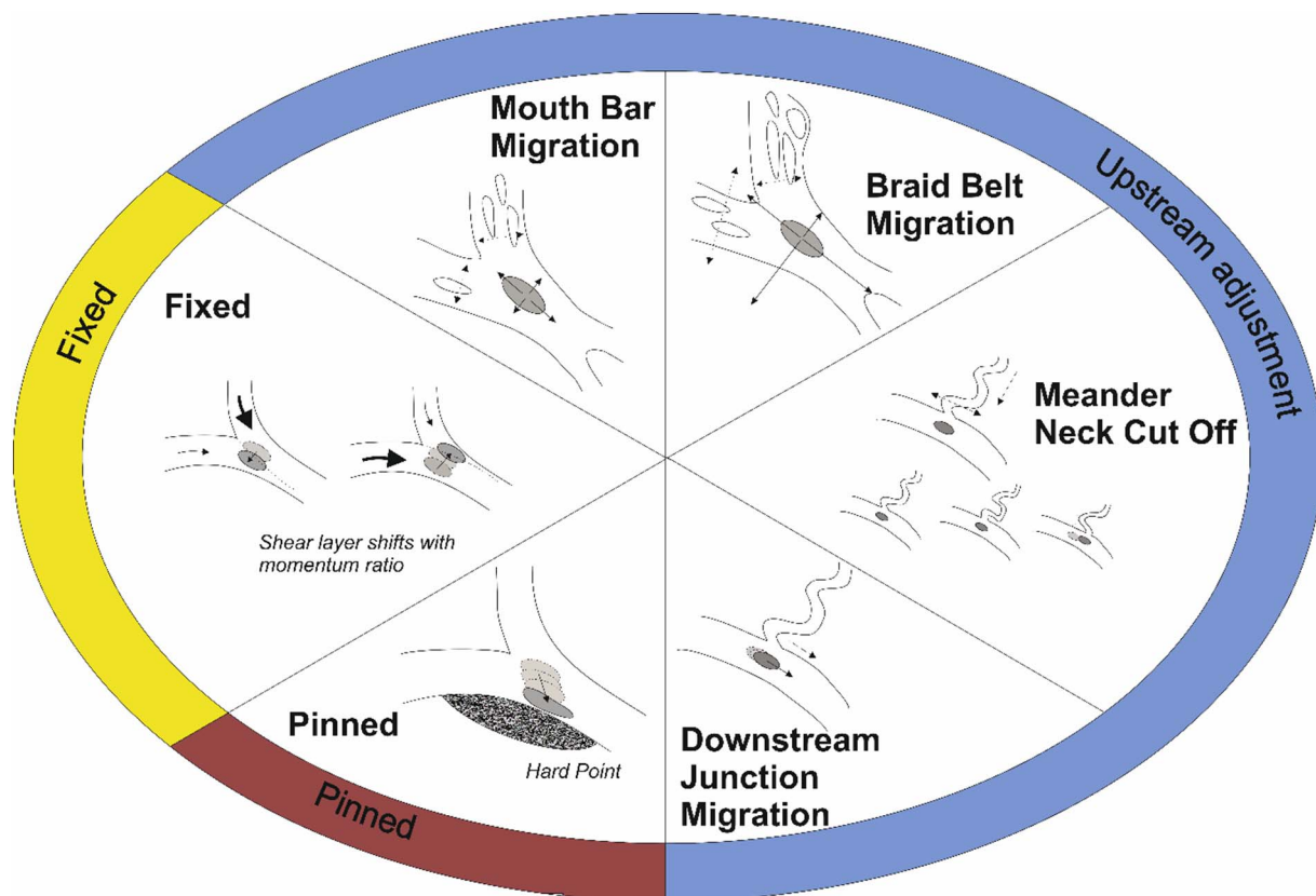
Fig. 14. A classification of confluence types based on analysis of Landsat imagery. See text for explanation.
