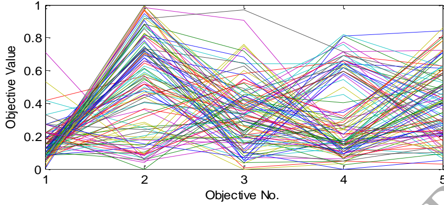
Fig. 9 Parallel coordinate plot of the Pareto front generated by MOTAMAQ at the rescheduling point t_r = 24.2 on sT20_dT10_E10_SK4-5.
