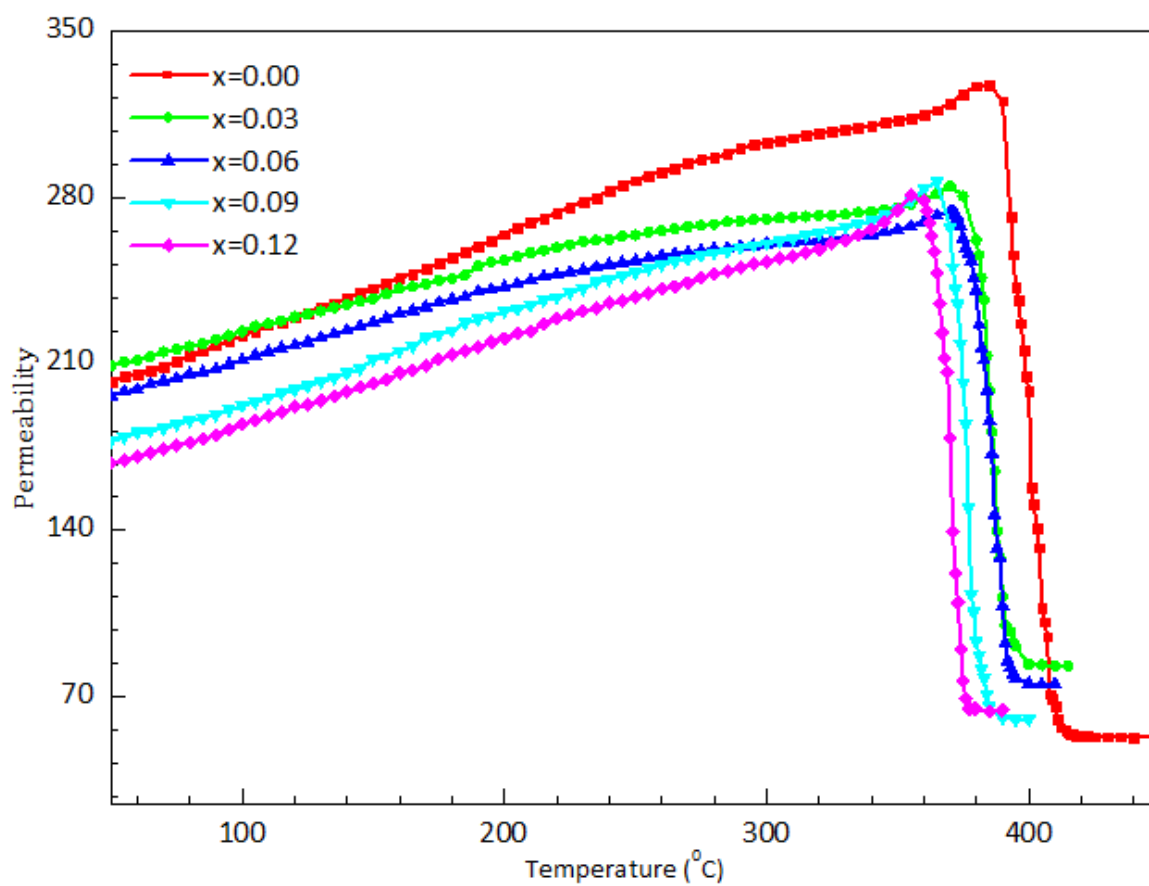
Fig. 6. Curie temperature estimation of Ni_{0.65}Zn_{0.35}Al_xFe_{2-x}O_4 ( x = 0, 0.03, 0.06, 0.09, 0.12 ) ferrites.
