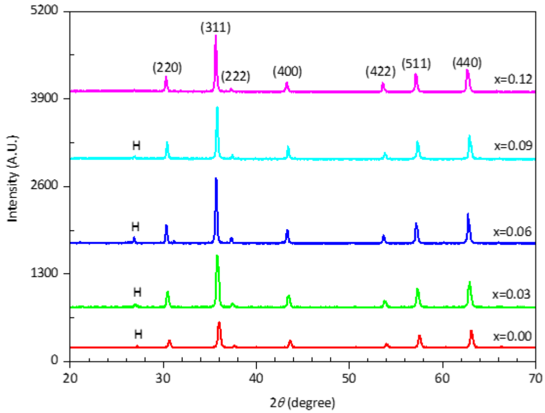
Fig. 1. XRD patterns of Ni_{0.65}Zn_{0.35}Al_xFe_{2-x}O_4 ferrites with different Al content.
