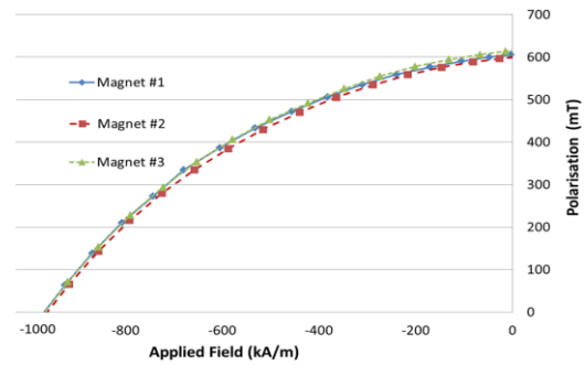
Fig.6. Demagnetization loops of three sample magnets taken at random from V2 set of magnets, measured using a closed-loop permeameter.
