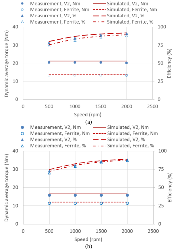
Fig.16. Dynamic torque and efficiency testing of the prototype motors with the recycled V2 and ferrite magnets. (a) Magnet at 40^\circ\text{C} and winding at 70^\circ\text{C} . (b) Magnet at 100^\circ\text{C} and winding at 120^\circ\text{C} .
