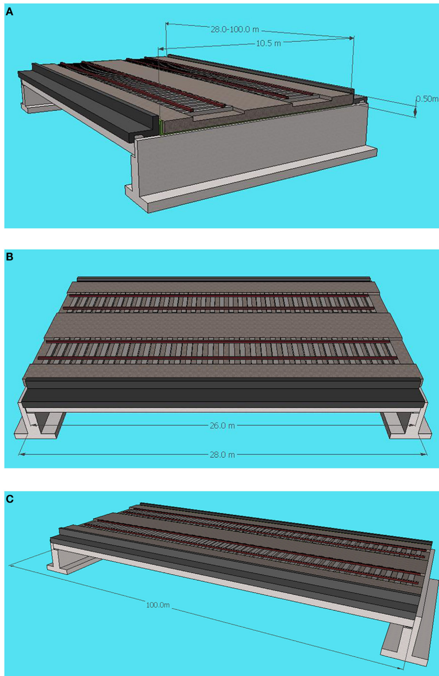
FIGURE 3 | Longitudinal sections of railway bridge. (A) bridge cross section; (B) longitudinal section of short span bridge; (C) longitudinal section of long span bridge.
