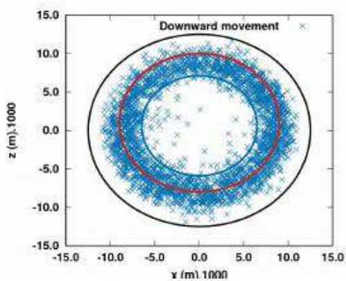
Downward motion near the wall
