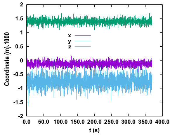
Figure 3: Measured position in a closed non-agitated vortex-shaker
