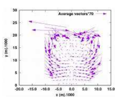
Time-averaged velocity vectors
