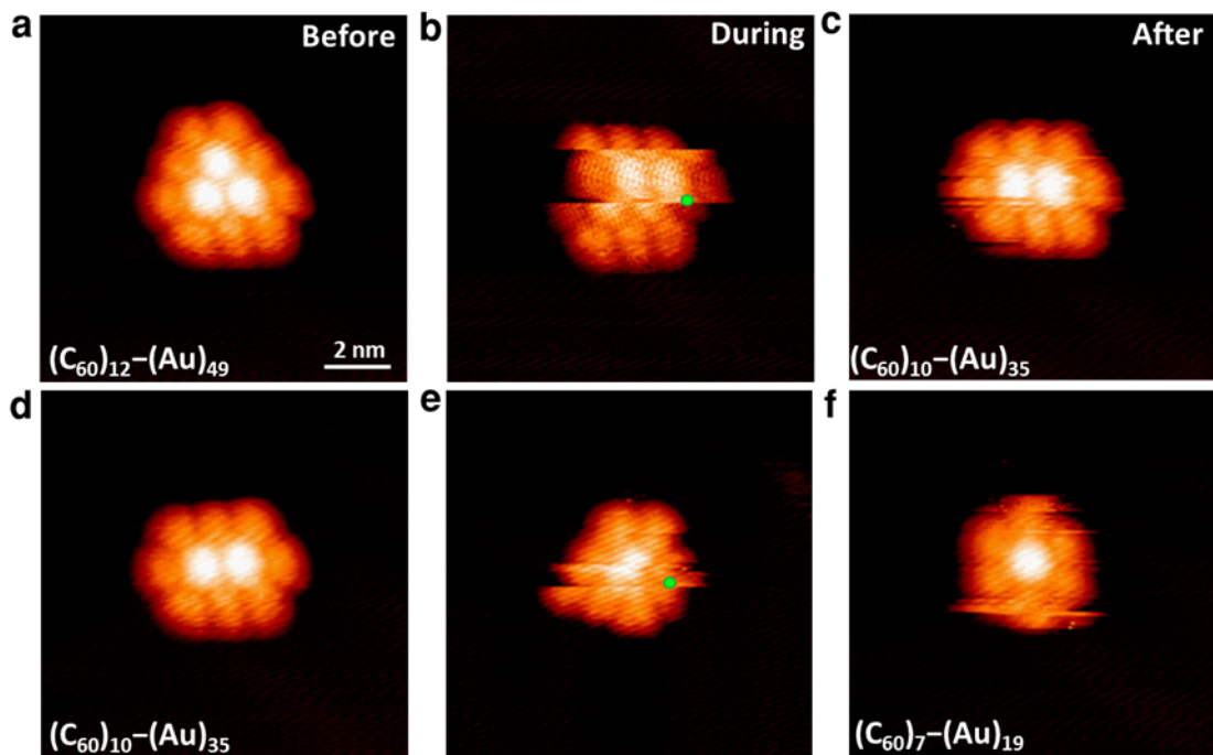
Figure 2: Tip-triggered cascade cluster transformation. (a-c) Transformation from (C_{60})_{12}-(Au)_{49} to (C_{60})_{10}-(Au)_{35} . (d-f) Transformation from (C_{60})_{10}-(Au)_{35} to (C_{60})_{7}-(Au)_{19} . Green dots in (b) and (e) indicate the locations where the tip is driven toward the C_{60} molecule.
