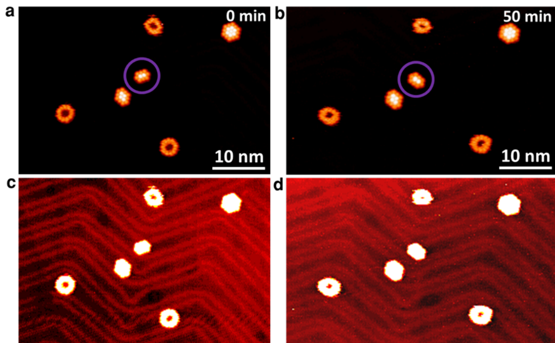
Figure 5: Flipping of a (C_{60})_{10}-(Au)_{35} cluster at room temperature without the application of an STM trigger. Image in (b) is taken 50 minutes after the image in (a). (c) and (d) The same images of (a) and (b), respectively, shown with enhanced contrast so that the locations of the clusters relative to the elbows of the herringbone reconstruction become visible.
