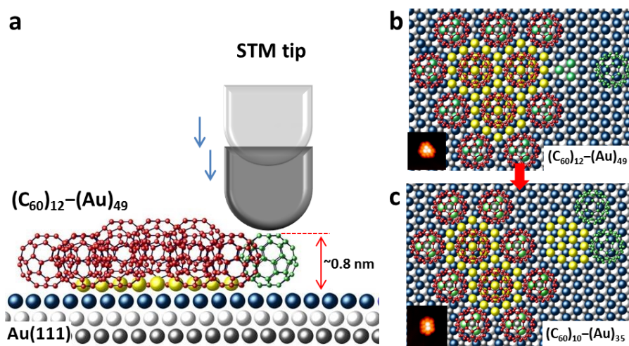
Figure 1: Schematic of the manipulation experiment. (a) The tip is located directly above a pre-selected molecule (green colored C_{60} ) at the edge of a cluster. It then moves towards the molecule by 1.2 nm. This is sufficient to detach the molecule from the cluster. A clean W tip is illustrated in the diagram although in reality the tip is likely to be coated with Au atoms. (b) As the tip withdraws, the displaced molecule either diffuses away or becomes attached to the tip. Green colored spheres represent first layer Au atoms that are in direct contact with C_{60} molecules. (c) The remaining atoms and molecules within the broken cluster re-organize to form a new magic number cluster by releasing excess C_{60} molecules and Au atoms.
