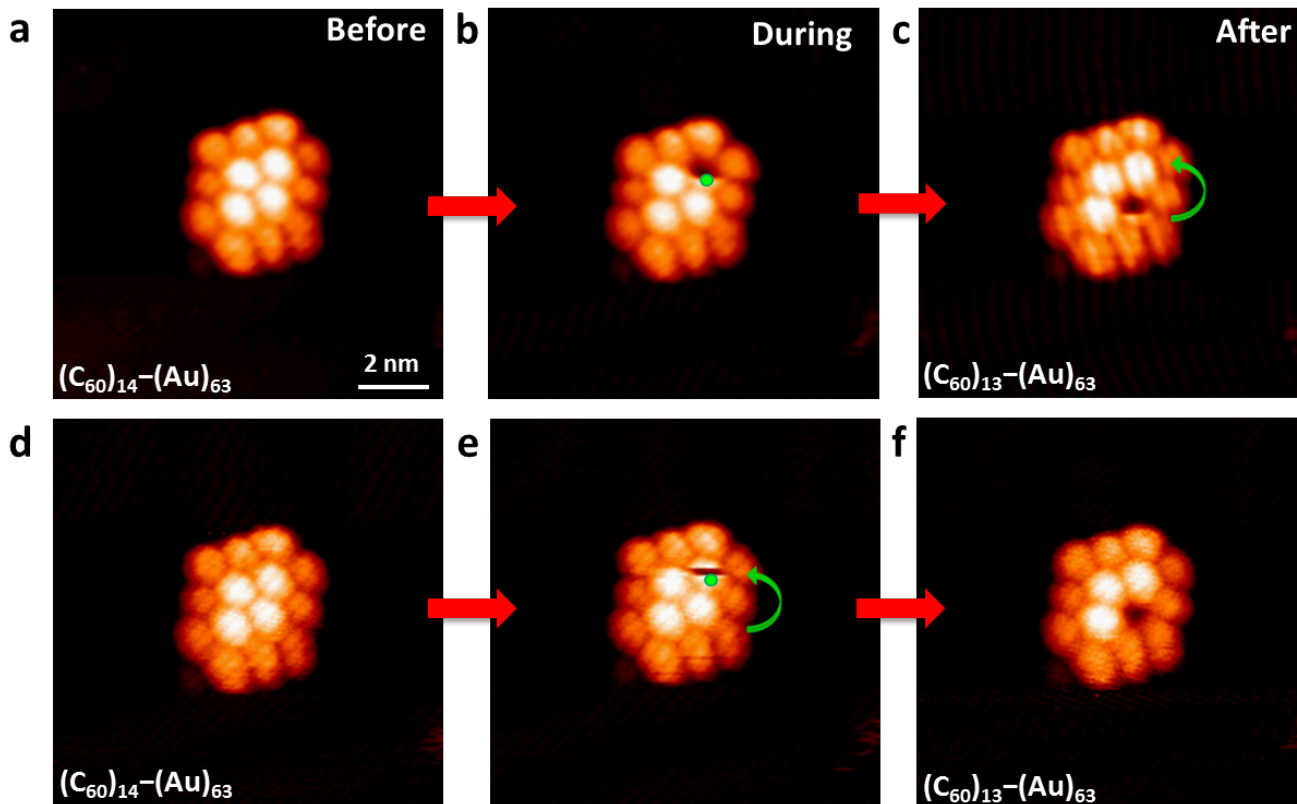
Figure 3: Single molecule extraction. (a-c) STM images showing the consequence of applying the manipulation trigger on a C_{60} molecule sitting above the Au island. The cluster here is (C_{60})_{14}-(Au)_{63} . (d-f) Similar manipulation performed on another (C_{60})_{14}-(Au)_{63} cluster. (b) and (e) Green dots indicate the locations where the triggers are applied. Green curved arrows indicate vacancy filling by diffusing C_{60} molecules.
