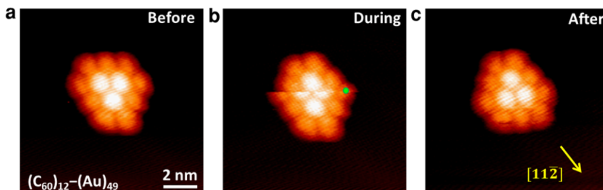
Figure 4: Tip-triggered rotation of a cluster. (a-c) STM images showing the flipping of a (C_{60})_{12}-(Au)_{49} cluster triggered by the STM tip. (b) Green dot indicates where the trigger is applied. The molecule targeted by the tip has not been removed. The cluster collectively changes its orientation.
