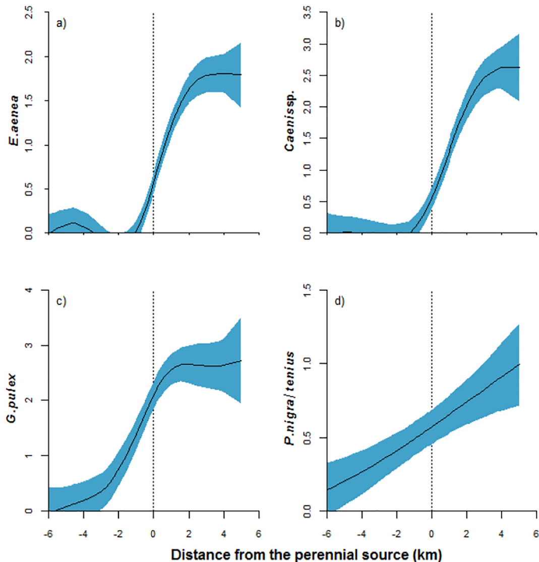
Fig. 5. The relationship between the \log_{10}(X + 1) transformed abundance of select taxa in relation to the distance from the perennial source outputted by the GAMM's. a) Elmis aenea ; b) Caenis . sp.; c) Gammarus pulex and d) Polycelis nigra .
