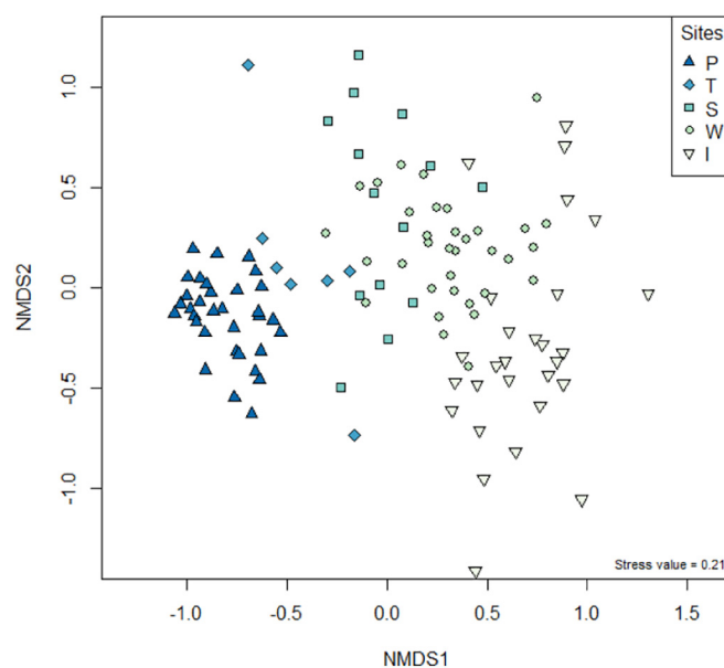
Fig. 3. NMDS plots of macroinvertebrates species-level community abundances between EHC groups. Triangles = 'Perennial'; Diamonds = 'Transitional'; Squares = 'Seasonal'; Circles = 'Winterbourne'; Inverted triangles = 'Intermittent'.
