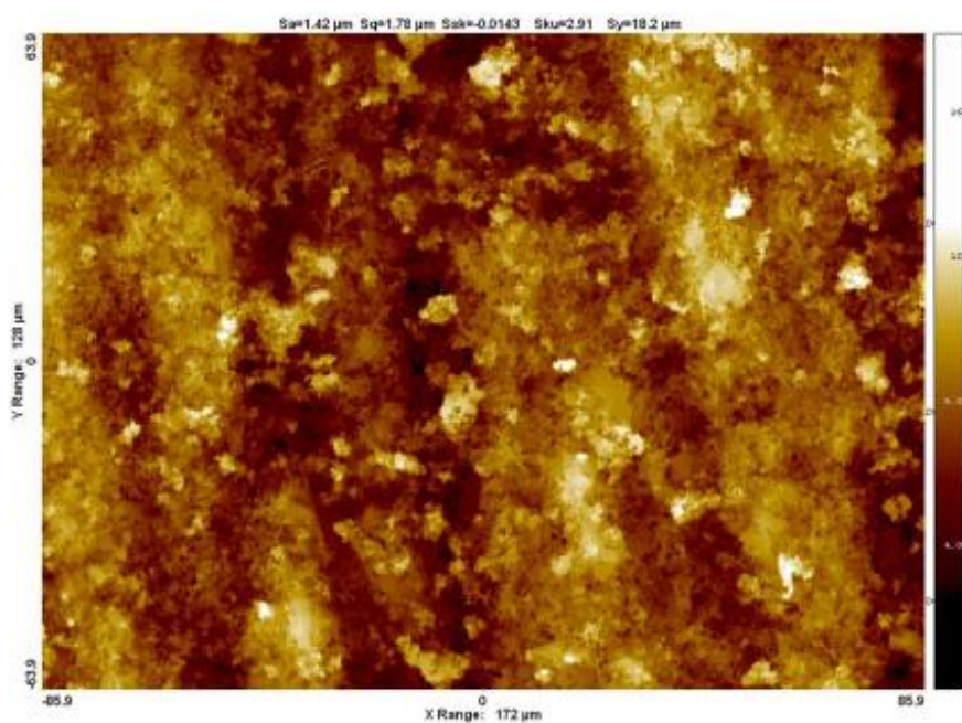
Figure 5: White light interferometry of the surface of a hydroxyapatite tablet prior to coating with peptides. The average roughness was S_a=1.42 \mu\text{m} .
