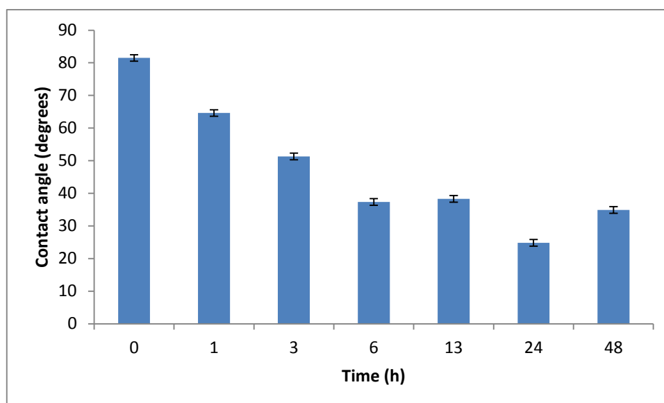
Figure 2: Water contact angle of Ti6Al4V etched using 30 wt % \text{H}_2\text{O}_2 aqueous solution for 0, 1, 3, 6, 13, 24 and 48 h; error bars correspond to standard deviation, with number of samples n=3 .
