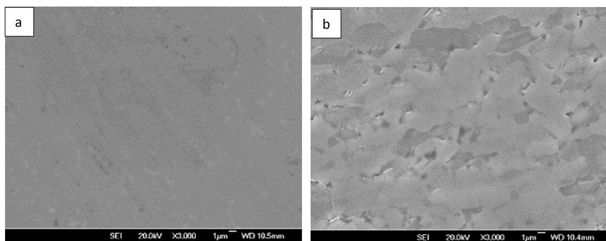
Figure 1: SEM micrographs X3000 of (a) Ti6Al4V mirror polished surface; (b) Ti6Al4V mirror polished surface after etching for 24 h.
