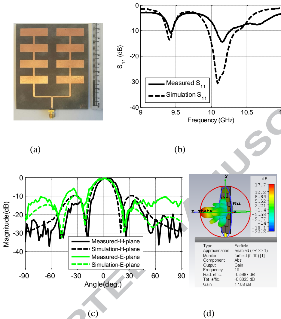
Fig. 6. Experiment results of 8-elements MPAA designed at 0.508mm thick PCB. (a) Fabricated prototype, (b) S_{11} , (c) 2-D FRP and (d) 3-D simulation FRP
