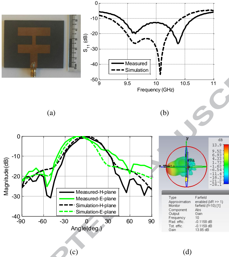
Fig. 2. Experiment results of 2-elements MPAA designed at 1.57mm thick PCB. (a) Fabricated prototype, (b) S_{11} , (c) 2-D FRP and (d) 3-D simulation FRP
