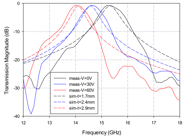
Fig. 11. Measured transmission magnitude for different voltages and comparison with simulated results.
