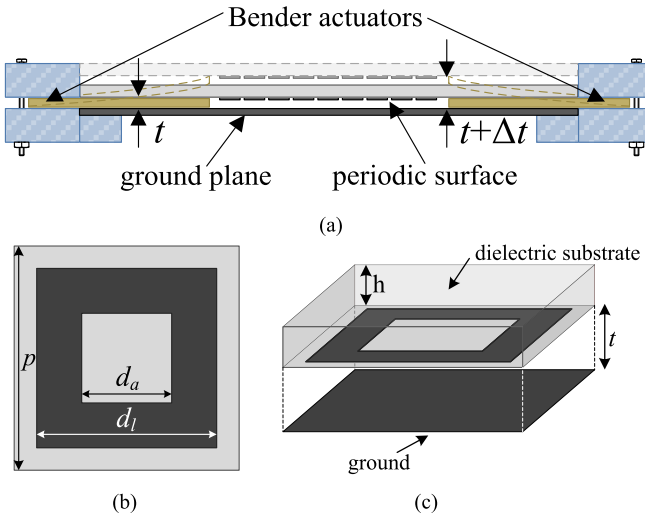
Fig. 1. (a) Proposed tunable HIS (dimensions are not to scale) and unit cell of the HIS array. (b) Top view. (c) Perspective.
