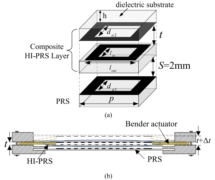
Fig. 6. (a) Unit cell of the multilayer FSmS. (b) Schematic of proposed tunable FSmS structure (dimensions are not to scale).
