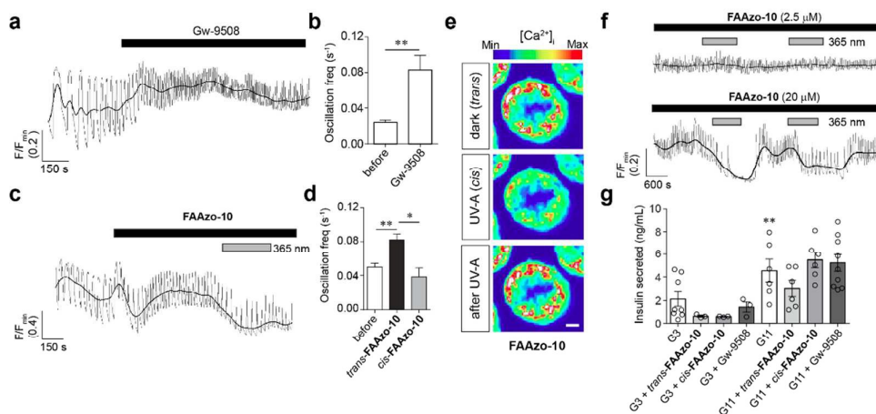
Fig. 7 FAAzo-10 enables optical control of [Ca^{2+}]_i oscillations in pancreatic islets. [Ca^{2+}]_i oscillations were stimulated by a high glucose concentration ( 11 \mu\text{M} , G11) and monitored in intact mouse islets using the fluorescent [Ca^{2+}]_i indicator Fluo-8. (a,b) The application of Gw-9508 ( 50 \mu\text{M} ) caused an increase in the [Ca^{2+}]_i oscillation frequency. Displayed as (a) a representative trace from a single islet and (b) the oscillation frequency averaged over multiple islets ( n = 6 recordings). (c,d) The application of trans - FAAzo-10 ( 20 \mu\text{M} ) also caused a marked increase in the oscillation frequency. Isomerization to cis - FAAzo-10 with 365 nm irradiation reversed this effect. Results are displayed as (c) a representative trace from a single islet and (d) the average oscillation frequency from multiple islets ( n = 5 recordings). (e,f) FAAzo-10 enabled optical control of \beta -cell [Ca^{2+}]_i oscillations at 20 \mu\text{M} , but not at 2.5 \mu\text{M} ( n = 4-5 recordings) (representative images cropped to show a single islet; scale bar = 25 \mu\text{m} ). (f) FAAzo-10 ( 20 \mu\text{M} ) did not afford a consistent effect on GISIS at [\text{glucose}] = 3 \mu\text{M} (G3) or G11. Gw-9508 ( 20 \mu\text{M} ) also did not affect secretion ( n = 3-8 assays using islets from at least 3 animals). Grey lines are raw traces (to show frequency effects), black lines are smoothed traces (to show amplitude effects). **denotes significance between G3 and G11. * P < 0.05 and ** P < 0.01 , ANOVA, with repeated measures as necessary. Error bars were calculated as \pm s.e.m.
