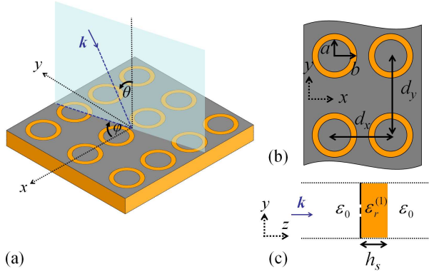
Fig. 1. (a) 2-D periodic structure with a rectangular array of coaxial annular apertures on a metallic screen backed with a dielectric slab. (b) Top view of a portion of the array structure. (c) Side view of a single unit cell.
