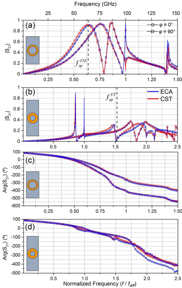
Fig. 5. Transmission coefficient for FSS and ET designs. ECA (blue line) and CST (red line) results are shown for vertical polarization, i.e. \varphi = 90^\circ (squares), and horizontal polarization, i.e. \varphi = 0^\circ (circles). (a) FSS - Magnitude. (b) ET - Magnitude. (c) FSS - Phase. (d) ET - Phase.
