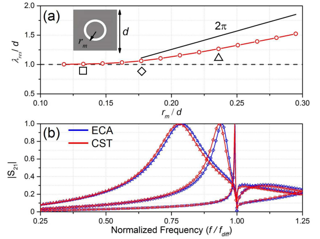
Fig. 3. (a) Resonant wavelength \lambda_{\text{res}} versus mean radius ( r_m ) normalized to the lattice period d for free-standing coaxial array of annular apertures with b/a = 1.3 and d = 1.5 mm. (b) Transmission coefficient results obtained by ECA (blue line) and CST (red line). [□] b = 0.25 mm ( r_m = 0.13d mm). [◇] b = 0.3 mm ( r_m = 0.177d mm). [△] b = 0.4 mm ( r_m = 0.236d mm).
