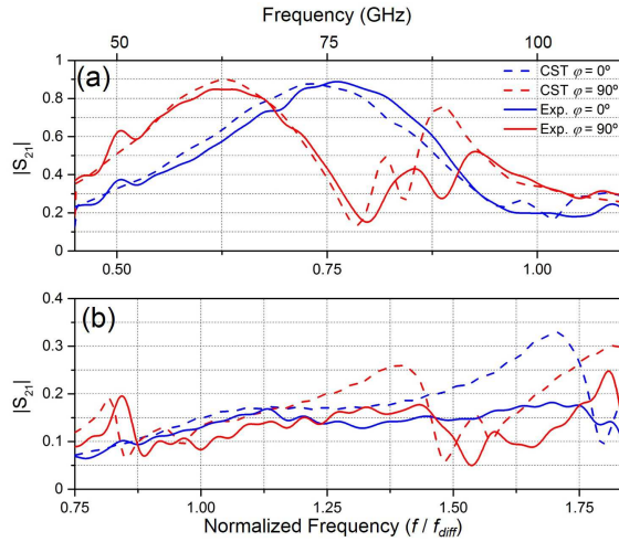
Fig. 9. Finite simulation and experimental results of fabricated samples for \varphi = 0^\circ and \varphi = 90^\circ incidence planes. (a) FSS prototype. (b) ET prototype.
