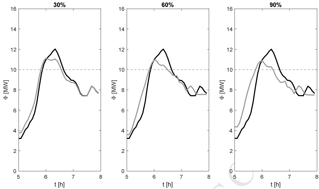
Fig. 8. Optimization results with external temperatures T= 5^{\circ}\text{C} -Objective Function 1-
