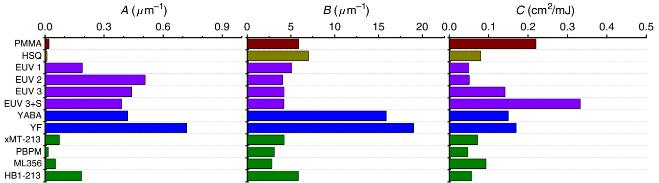
Fig. 6 Summary of the measured Dill parameters: bleachable coefficient A , unbleachable coefficient B , and exposure rate constant C of resists investigated in this work.
