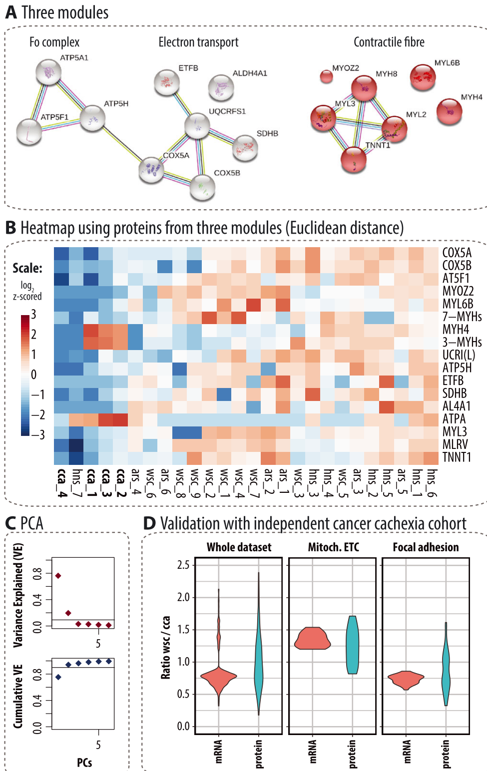
Figure 2 Third-order data analysis. (A) Protein–protein interaction analysis of highly regulated proteins with statistical significance resulted in three modules distinguishing cachexia from all other patients or healthy elderly. (B) Heatmap of proteins representing protein clusters identified above (ars: age-related sarcopenia, cca: cancer cachexia, hns: healthy non-sarcopenic, wsc: weight-stable cancer). (C) Principle component analysis of protein signature demonstrating that three proteins would be able to explain the variance differentiating between cachexic and all other patient groups. (D) Cross validation of identified protein modules by alternative protein abundance measurements on independent cohort. 32
