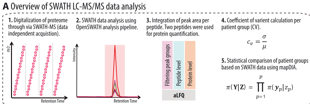
Figure 1 Proteomics data. (A) Overview of computational analysis of liquid chromatography coupled to tandem mass spectrometer (LC-MS/MS) data acquired in SWATH mode. First, the mass spectrometer acquires the m/z ratio in a data independent fashion. Areas under the curve of co-eluting transitions are the basis for peptide quantification. Automatically annotated peptides are filtered based on quality scores and give rise to protein quantification, which are further analysed by mathematical and statistical algorithms. (B) Heatmap of all proteins quantified per patient (ars: age-related sarcopenia, cca: cancer cachexia, hns: healthy non-sarcopenic, wsc: weight-stable cancer). (C) Violin plots of coefficient of variance (CV) per patient groups. (D, E) Volcano plots of statistical significance analysis focusing on cachexic vs. other patient groups.
