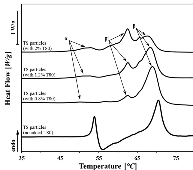
Fig. 6. DSC melting thermograms of dispersions with varying concentrations of Tween 80. The curve of the dispersion without surfactant is provided for comparison. All samples were melted from 20 to 85 °C at 1.2 °C/min. The lipid fraction is constant at 2.5 wt/wt%.
