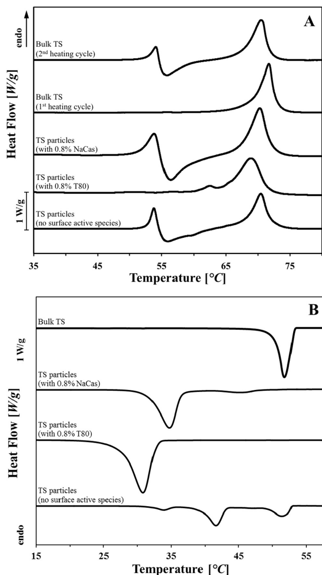
Fig. 5. DSC (A) melting and (B) crystallisation curves (scan rate 1.2 °C/min) of bulk tristearin (TS), of a 2.5% particulate tristearin dispersion without any surfactant and of 2.5% tristearin dispersion produced in the presence of 0.8% Tween 80 (T80) and 0.8% sodium caseinate (NaCas), measured after preparation of the dispersions. The curves are normalised for the sample weight and the amount of crystalline material present, and displaced along the ordinate for better visualisation.
