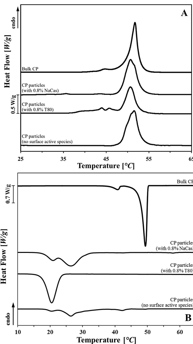
Fig. 7. DSC (A) melting and (B) crystallisation curves (scan rate 1.2 °C/min) of bulk cetyl palmitate (CP), of a 2.5% particulate CP dispersion formed in the absence of surface active species and of 2.5% CP dispersion formed using 0.8% Tween 80 (T80) and 0.8% sodium caseinate (NaCas), measured after preparation of the dispersions.
