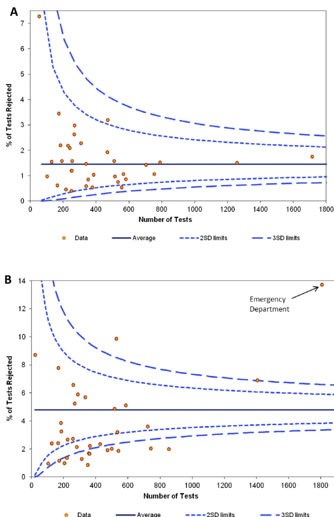
Fig. 1. A: A funnel plot of haemoglobin rejection rate by clinical area. B: A funnel plot of potassium rejection rate by clinical area.
