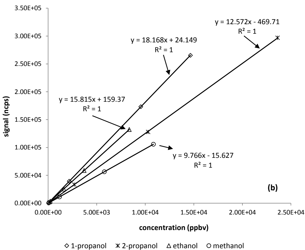
Figure 1. Calibration curves for 1-propanol, 2-propanol, ethanol and methanol at physiologically representative concentrations; data acquired using SIFT-MS (a) and PTR-MS (b).
