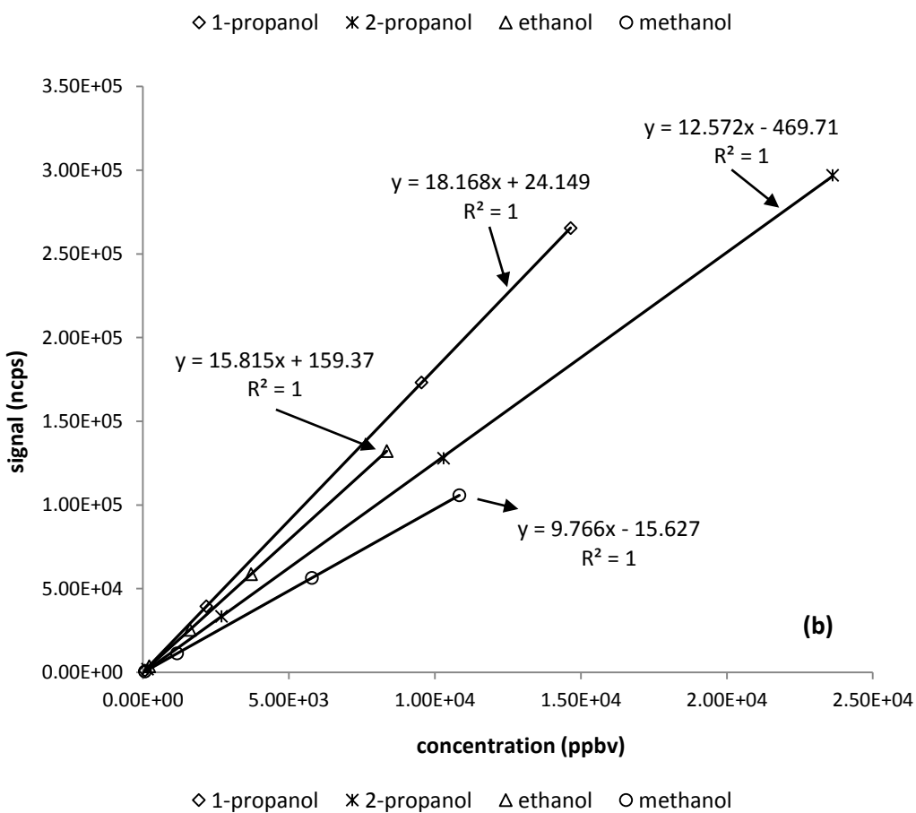
Figure 1. Calibration curves for 1-propanol, 2-propanol, ethanol and methanol at physiologically representative concentrations; data acquired using SIFT-MS (a) and PTR-MS (b).
