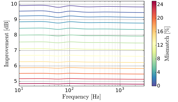
FIG. 5: The figure shows the effect of mode-mismatching the interferometer to the squeezer and the filter cavity. We see a broad-frequency band decrease in improvement that is similar to an optical loss.
