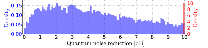
FIG. 11: The figure shows the "probability density" for obtaining a certain quantum noise reduction when mixing a squeezed vacuum with pure vacuum (blue) and when mixing two squeezed vacuum fields (red). The squeeze angles have, for both distributions, been optimized to minimize the noise.
