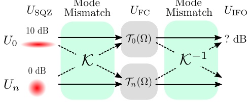
FIG. 7: The figure shows the effect of mode-mismatching the filter cavity to the squeezer and the interferometer. The noise fields in the two spatial modes mix twice, with a frequency and mode dependent rotation of the squeeze angle in between due to the filter cavity. Since the squeezer and the interferometer are mode matched, the two mixing operations are the inverse of each other.
