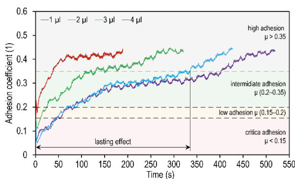
Fig. 4. Friction curves for various quantities of FM.
