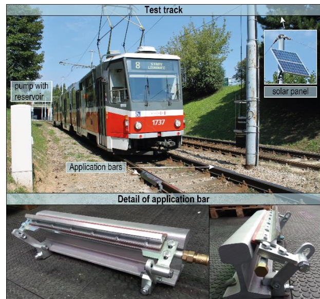
Fig. 3. Detail of new-developed off-board system.
