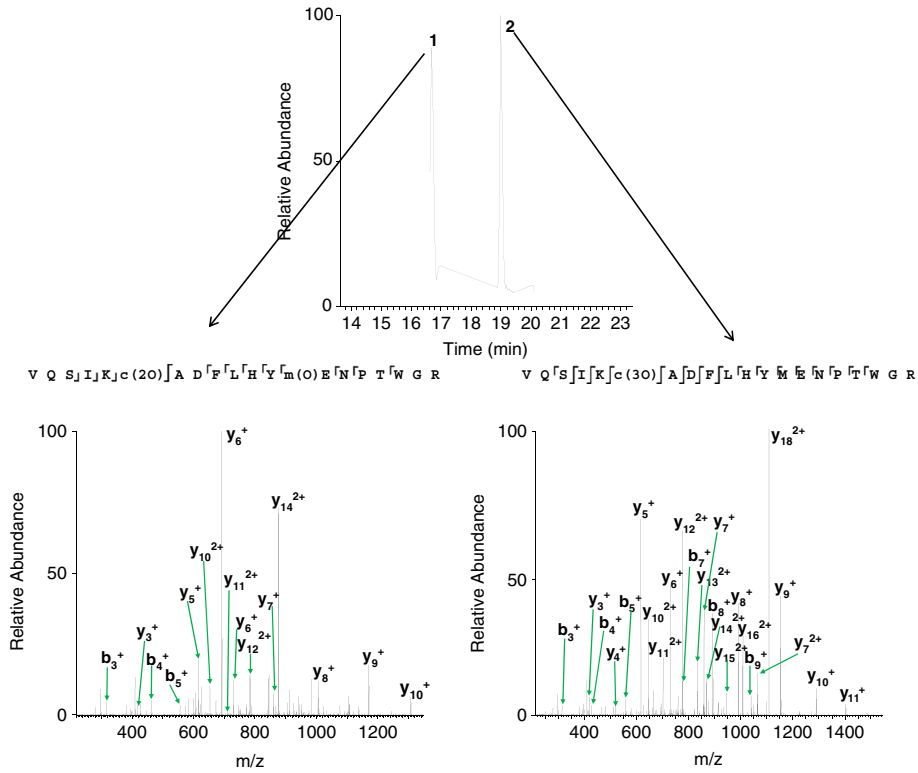
Figure 3. Extracted ion chromatogram ( m/z 815.0426, [VQSIKCADFLHYMENPTWGR +3O]) obtained following LC CID MS/MS and the two corresponding CID MS/MS spectra at retention times 16 min 45 s and 19 min. Observed fragments are summarized on the peptide sequences, inset. Lower case denotes modified amino acid residues
