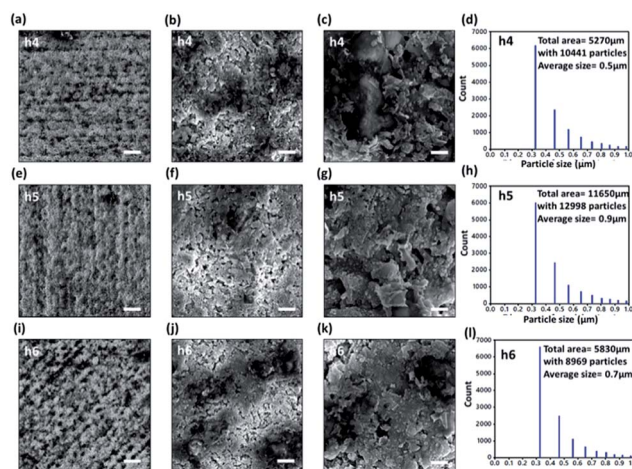
Fig. 3 SEM images of the laser-patterned nanoripples (h4, h5 and h6). (a, e and i) 1000× magnification. Scale bar = 25 μm. (b, f and j) 20 000× magnification. Scale bar = 2.5 μm. (c, g and k) 35 000× magnification. Scale bar = 1 μm. (d, h and l) Histograms showing the particle size distribution of h4, h5 and h6 samples.
