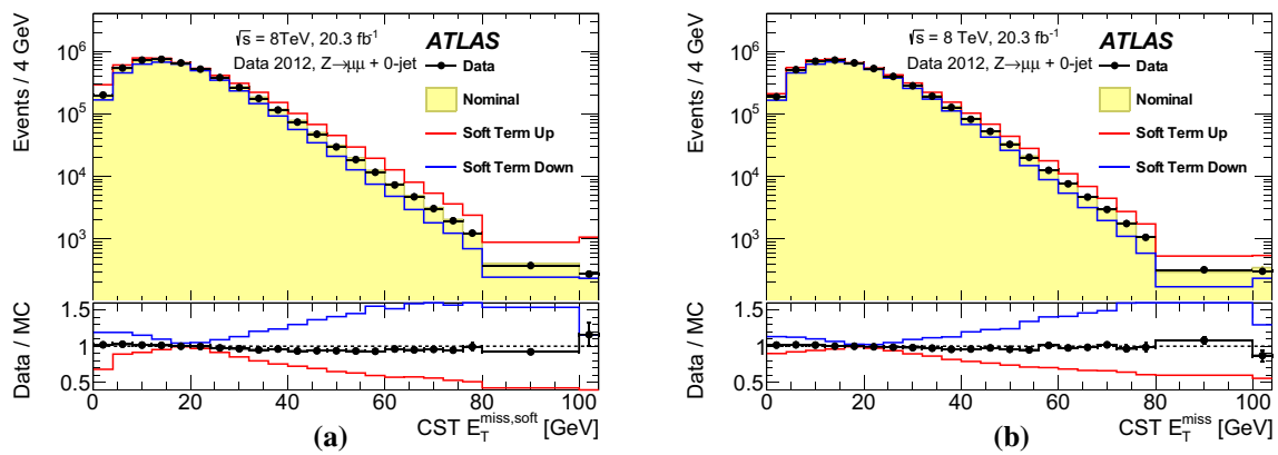
Fig. 25 Distributions of a E_T^{miss,soft} and b E_T^{miss} with the CST algorithm. Data are compared to the nominal simulation distribution as well as those resulting from applying the shifts/smearing according to the scale and resolution systematic uncertainties on the E_T^{miss,soft} . The
