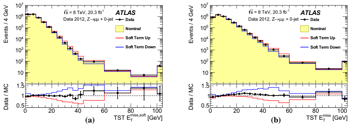
Fig. 26 Distributions of a E_T^{miss,soft} and b E_T^{miss} with the TST algorithm. Data are compared to the nominal simulation distribution as well as those resulting from applying the scale and resolution systematic uncertainties to the E_T^{miss,soft} and adding the variations in quadrature,
