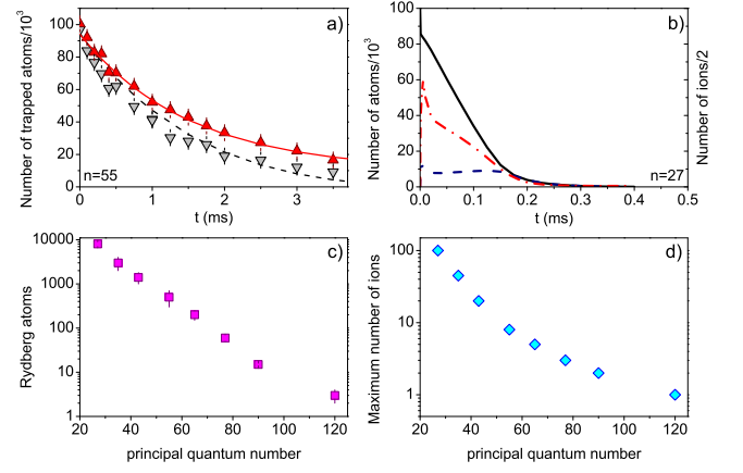
FIG. 3. (Color online) a) Typical decay measurements in (downpointing triangles) and out of resonance (uppointing triangles) together with the curves obtained as solutions of the rate equation system (2) for the 55s state. b) Time evolution of total number of trapped atoms (solid line), Rydberg atoms (dashed) and ions (dashed-dotted) for the 27s state. c) Calculated average number of Rydberg atoms present as a function of n . d) Calculated maximum number of ions present as a function of n .
