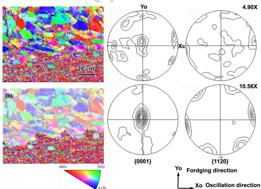
Fig. 5 EBSD results of one side of TMAZ in a Ti64 weld, (a) \alpha phase orientation map with regard to Z0 direction with the \{0001\}_\alpha and \{11\bar{2}0\}_\alpha pole figures; (b) orientation map without primary \alpha with the \{0001\}_\alpha and \{11\bar{2}0\}_\alpha pole figures. The contours in all pole figures show increment of 1.1 times random.
