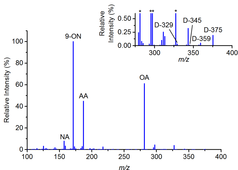
Figure 3: Mass spectrum of partially oxidized oleic acid aerosol acquired using EESI-MS. The initial particle-phase products of oleic acid ozonolysis, nonanoic acid (NA), 9-oxononanoic acid (9-ON) and azaleic acid (AA) are detected along with unreacted oleic acid (OA). The inset graph is an expansion of the region above m/z 275 which includes assignments of dimer products resulting from the reaction of primary products with Criegee intermediates. m/z intensities will be a function of both analyte concentration and ionization efficiency; we relate relative intensity changes to relative concentration changes in the aerosol, but note that the most intense peaks are not necessarily the most abundant aerosol species. The peaks marked (*) are cut off on the expanded scale.
