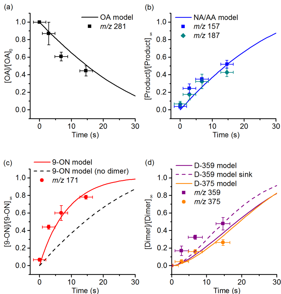
Figure 5: Modelled concentrations as a function of time for (a) oleic acid (OA), (b) nonanoic acid (NA) and azaleic acid (AA), (c) 9-oxononanoic acid (9-ON) and (d) dimer products, dimer-359 and dimer-375. EESI-MS measurements with 8 ppm ozone are included as discrete points and both model and experimental results are scaled to aid comparison. The model shows a close fit to the measured OA (a) and primary product ((b) and (c)) data, and reasonable agreement for the dimer products (d). NA and AA (b) have the same modelled time dependence owing to the symmetry of the mechanism (Figure 2). The dashed line in (c) represents a simulation with the dimer chemistry switched off, and the dashed line in (d) includes a unimolecular sink for D-359 ( k_{\text{sink}} = 0.01 \text{ s}^{-1} ) as a proxy for further dimer reactions.
