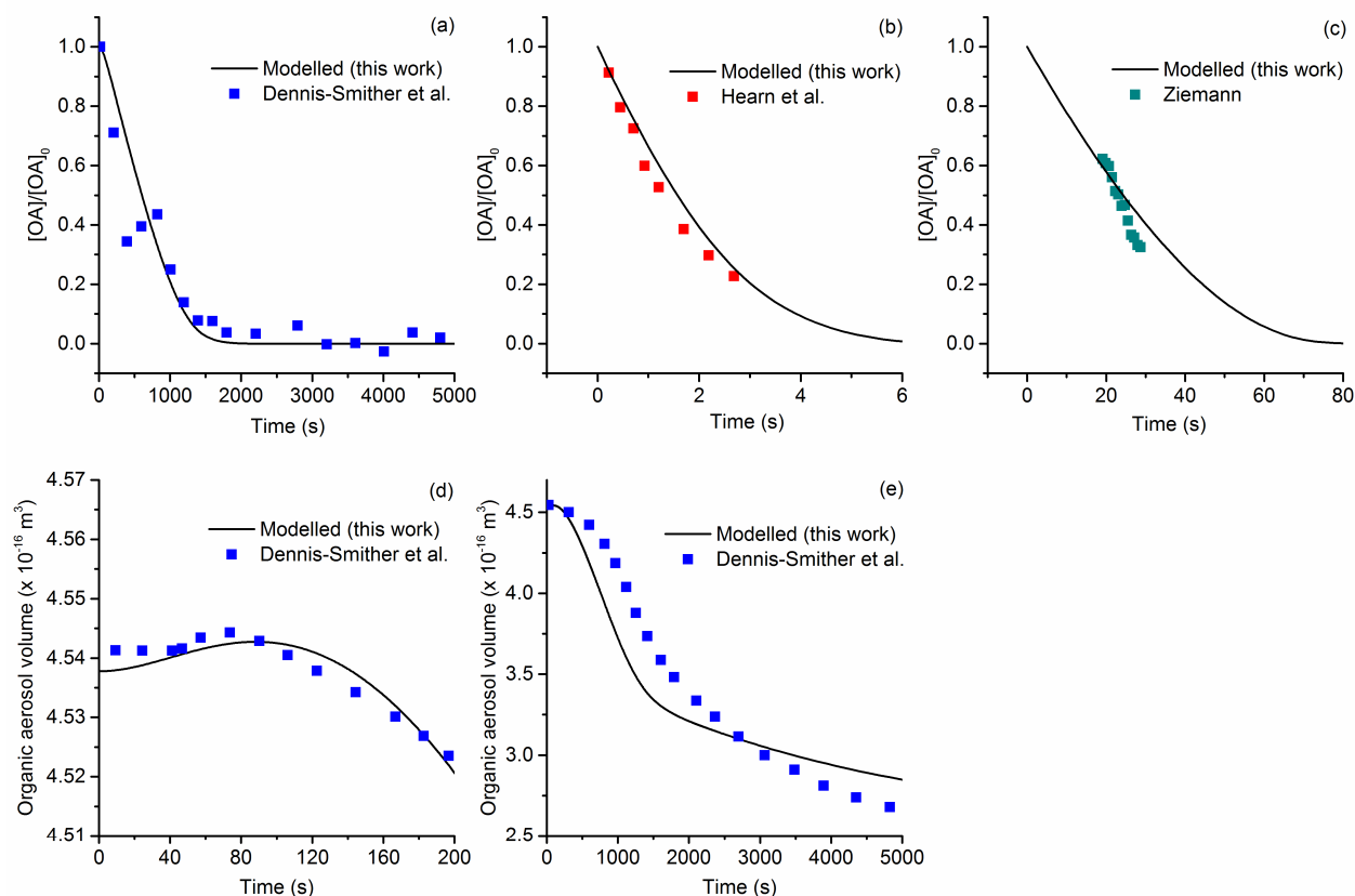
Figure 6: Model simulations compared with observations of oleic acid loss for (a) Dennis-Smith et al. , [2012], (b) Hearn et al. , [2004] and (c) Ziemann [2005]. We also simulate the single particle volume change of Dennis-Smith et al. , (d) at the start of ozonolysis and (e) over the experiment timescale. The model parameters were as for the base case (Table S1) with changes according to the experiment-specific parameters in Table 2. For the simulation in (b), precision and accuracy checks were turned off from Mathematica's NDSolve routine to allow the model to execute. The experimental data in (c) were obtained directly from P. Ziemann since the Figure presented in Ziemann [2005] contains a small error. These data were offset in time to coincide with the simulated curve and account for the mixing period in the chamber experiment.
