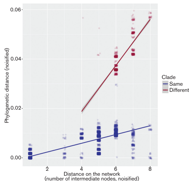
Fig. 2. Scatterplot showing the relationship between the phylogenetic distance and the distance between cases on the trace-back network, after accounting for the existence of two distinct genetic clades in sampled isolates. Each dot represents a pairwise comparison between two cases. Data have been slightly noisified to better visualise overlapping points. Dots are colored according to clade memberships, with pairs of isolates from the same clade in blue, and from different clades in red. Lines indicate predictions of a linear model using different slopes for each group.
