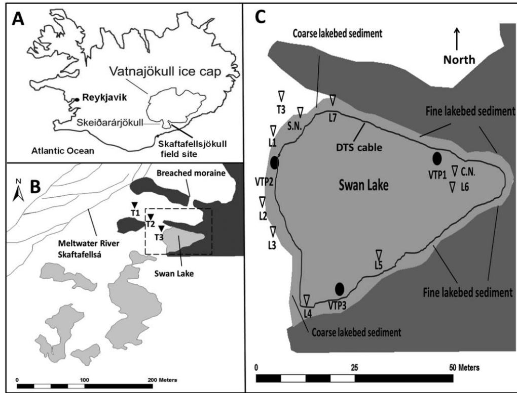
Figure 1. Map of the field site in Iceland (A), the proglacial zone of the Skaftafellsjökull glacier (B), and details of study area Swan Lake (dashed box in B, C). Swan Lake has no outlet stream. Inverted triangles denote piezometers, and circles denote the location of the Vertical Temperature Profiles (VTP). The location and deployment of the Fiber-Optic Distributed Temperature Sensor (FO-DTS) cable is shown as a black curve. Clay nest (C.N.) and Sand Nest (S.N.) denote 12-mm diameter piezometer nests within the respective sediment. L1–7 denote piezometers with internal diameter of 12 mm. T1–3 denote shallow boreholes with internal diameter of 22 mm.
