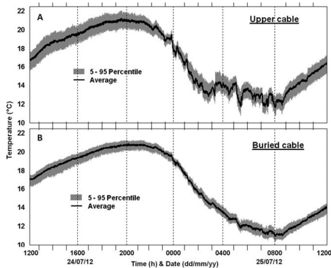
Figure 3. Mean and 5 th and 95 th percentile temperatures (T) for lake-bed sediment (upper cable) (A) and 10 cm depth within the lake-bed sediment (buried cable) (B) recorded during the Fiber-Optic Distributed Temperature Sensor (FO-DTS) temperature surveys.
