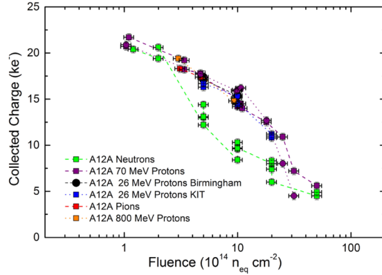
Figure 8. Measurements of collected charge at 500 V for sensors irradiated at the University of Birmingham and other facilities. Comparison data reported in Ref. [13]
