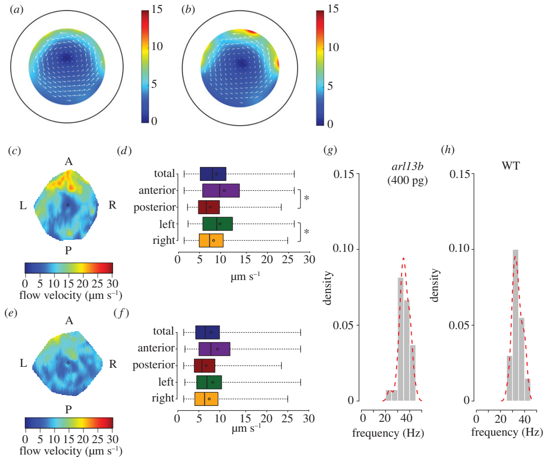
Figure 2. Predicted and observed flow patterns for long cilia. (a) Predicted flow map from WT embryos. (b) Predicted flow map to arl13b -injected embryos. The pseudocolour scale represents flow speed, where red represents high speed versus low speed in blue. (c,d) Experimental data for WT embryos shown as heat map of flow speed (c) and as a box plot for quantification (d). (e,f) Experimental data for arl13b-gfp overexpressed embryos (injected with 400 pg of arl13b-gfp mRNA per embryo) represented as a heat map of flow speed (e) based on the same dataset used to generate the box plot (f). The colour scale represents flow speed in \mu\text{m s}^{-1} , where red represents high speed versus low speed in blue. Box plots for instantaneous flow speed were based on measurements at different locations of the KV based on 243 tracks for seven WT embryos and 525 tracked native particles in a total of seven embryos overexpressing Arl13b-GFP. (g,h) Cilia beat frequency average in WT and Arl13b-GFP overexpressing embryos from a total of 30 motile cilia for each condition. Source data in http://dx.doi.org/10.5061/dryad.m541q [30].
