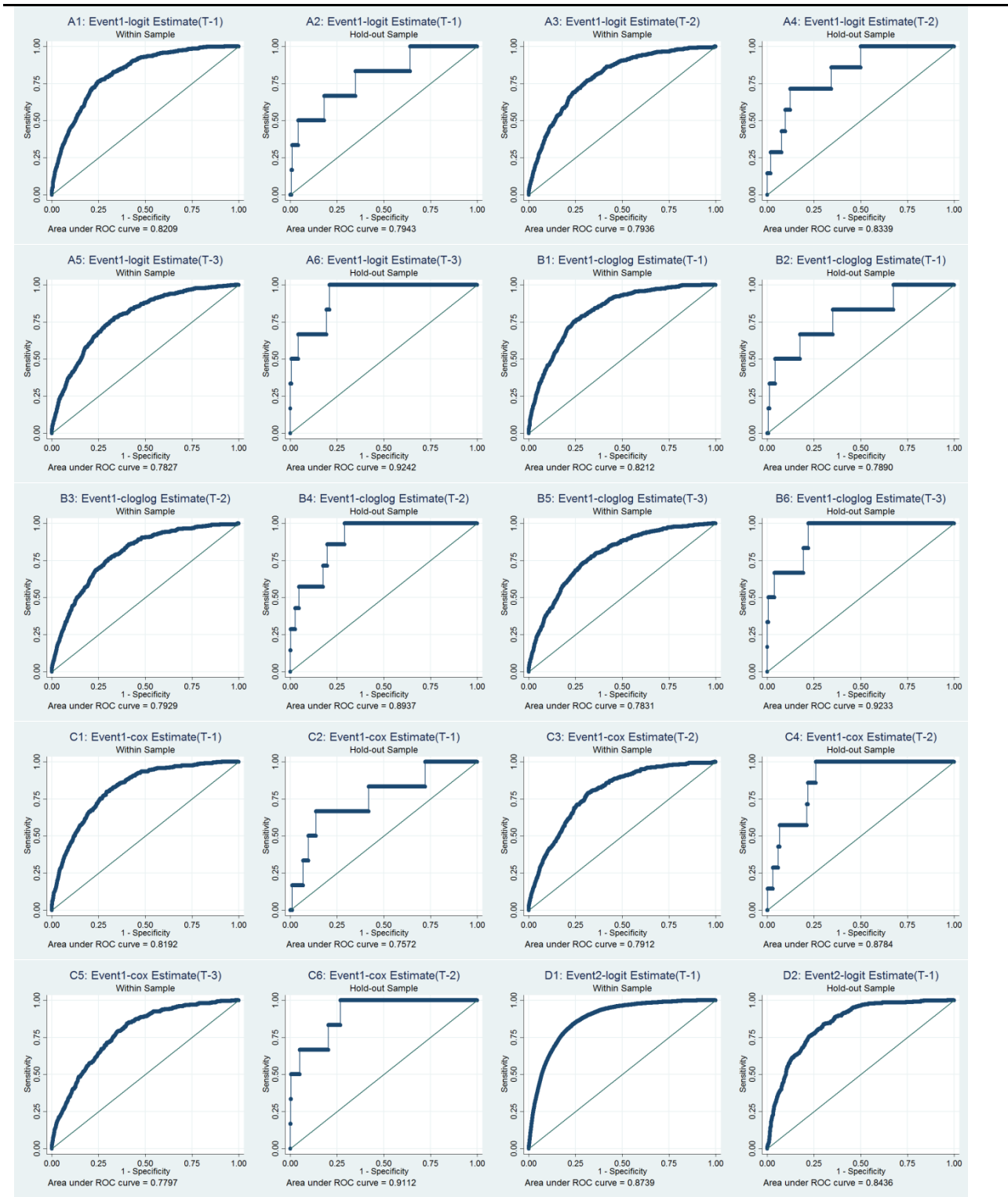
Figure 2: Table of Area under ROC curves
