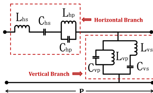
Fig. 1. Equivalent circuit model of one asymmetric ECRLH unit cell.
