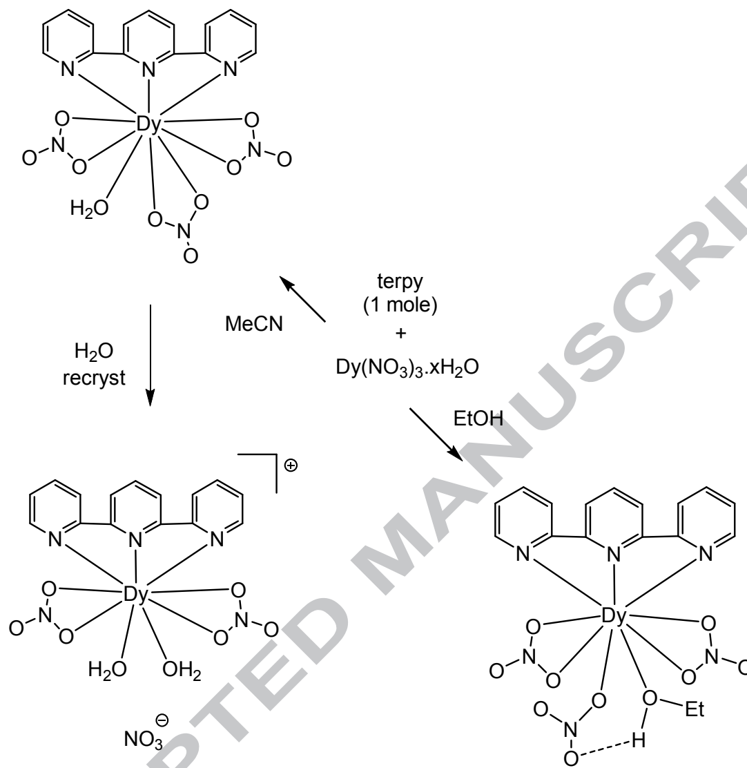
Fig. 15. The effect of solvents on the “[Dy(terpy)(NO 3 ) 3 ]” system
