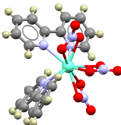
Fig. 4. The structure of the 10-coordinate [\text{Eu}(\text{bipy})_2(\text{NO}_3)_3] complex [34]
