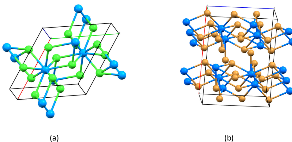
Fig. 1. (a) The structure of \text{UCl}_3 showing the 9-coordinate U atoms. (b) The structure of \text{PuBr}_3 showing the 8-coordinate Pu atoms.
