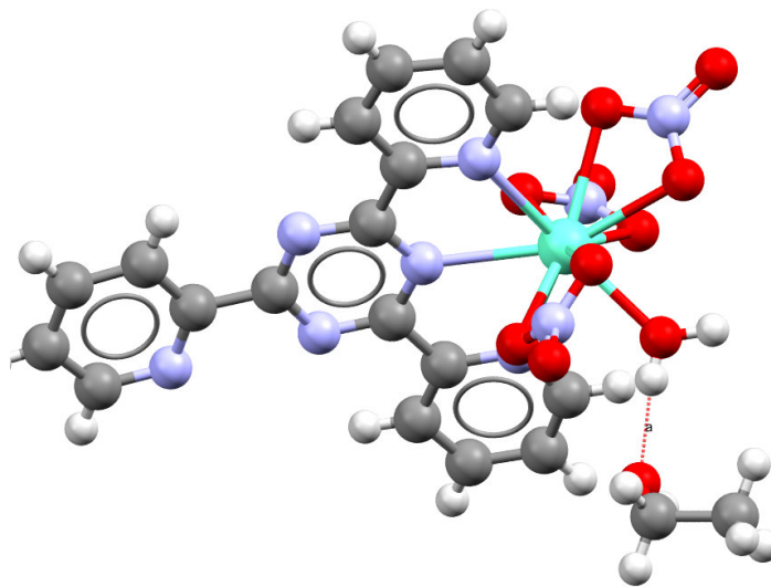
Fig. 6. The structure of [\text{Eu}(\text{tptz})(\text{NO}_3)_3(\text{H}_2\text{O})] \cdot 2\text{C}_2\text{H}_5\text{OH} as an exemplar of the series [\text{Ln}(\text{tptz})(\text{NO}_3)_3(\text{H}_2\text{O})] \cdot 2\text{C}_2\text{H}_5\text{OH} . A hydrogen bonded ethanol molecule is included to illustrate the importance of the solvent in the crystallisation process.
