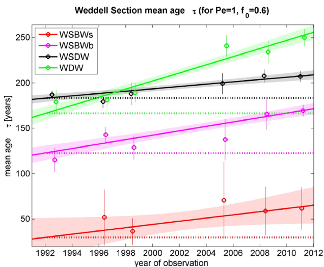
Fig. 23 Time series of ages in WDW, WSDW, and WSBW (left) and C ant at the Weddell Sea section (location see Fig. 18). The stippled lines show the expected trends in these water masses when assuming a steady state
