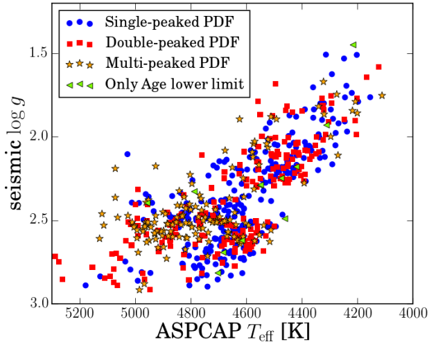
Fig. 8. Seismo-spectroscopic Hertzsprung-Russell diagram of the CoRoGEE stars, with the symbols indicating the qualitative behaviour of the age PDFs, as described in the legend.
