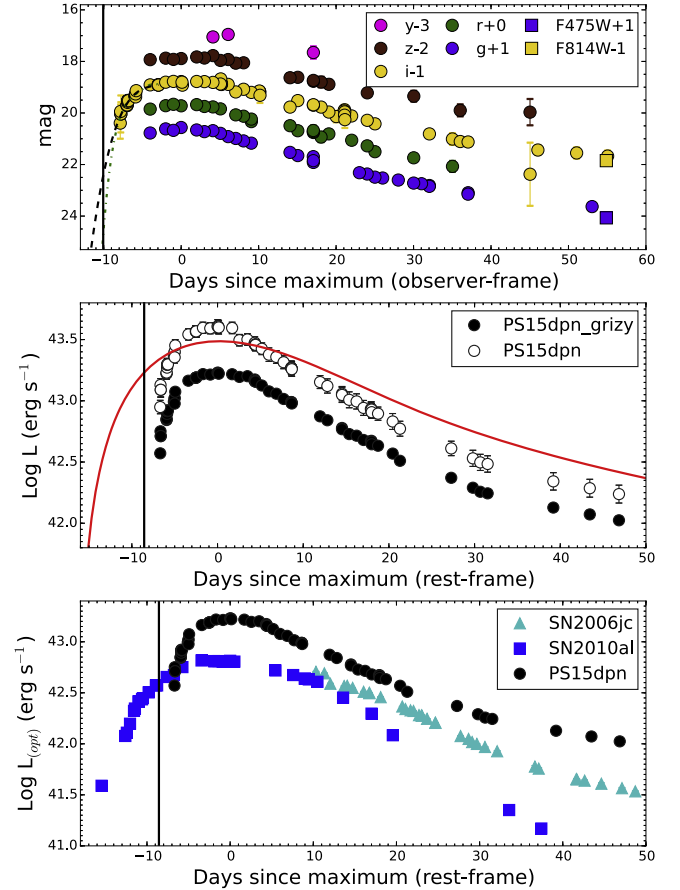
Figure 2. Upper: PS1 light curve of PS15dnp. Circles are PS1 and square symbols are from HST . The black dashed line is a third order fit and the green dotted-dashed is a fourth order fit (each fit to the first six epochs). The vertical black line indicates the time of the GW151226 event. Middle: bolometric luminosity calculated with grizy P filters only (see Insera et al. 2016 for details) and a full bolometric light curve estimated from a blackbody extrapolation between 0.2 and 2.5 \mu m. A simple Arnett model, as described in Insera et al. (2013), is shown for the latter, with input parameters: E_{\text{exp}} = 5 \times 10^{51} erg, M_{\text{ej}} = 1.9 M_{\odot} , M_{\text{Ni}} = 1.7 M_{\odot} . This simply indicates that a ^{56}\text{Ni} model is a poor fit and that type Ibn are not well explained by radioactive powering. Lower: comparison with two well observed SN Ibn (Pastorello et al. 2007, 2015).
