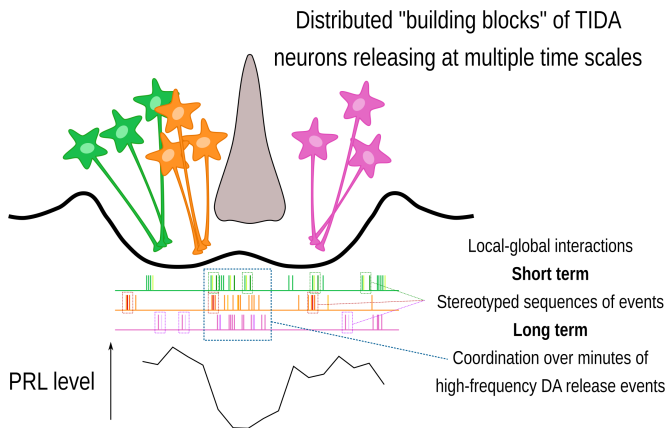
Fig. 4. Schematic of the brain-pituitary dialog proposed to underlie hypothalamic dopaminergic control of pituitary prolactin secretion. Illustrated are three sub-sets of hypothalamic TIDA neurons (colored in green, brown and magenta), which each locally release dopamine (DA) at the median eminence level (where the first loop of portal capillaries reside). Local DA release events are organized in the frequency domain (0.001 Hz-10 Hz) and recur as sequences. Local-global integration across the median eminence coordinates high frequency DA release events within the minutes range. This allows the build-up of DA in the portal blood required to efficiently inhibit pituitary prolactin secretion.
