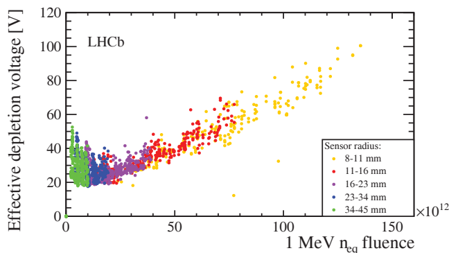
Fig. 6. The effective depletion voltage versus fluence for all VELO sensors up to the end of LHC Run 1 at 3.4 \text{ fb}^{-1} delivered integrated luminosity. 29
