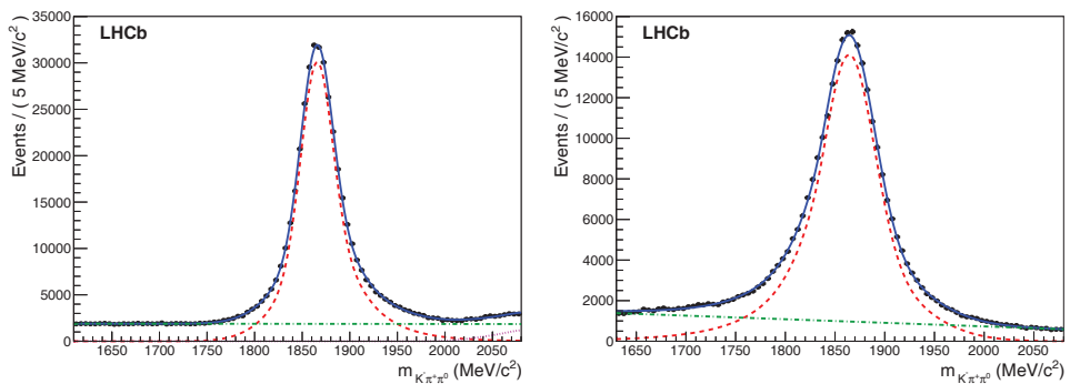
Fig. 31. Mass distributions of reconstructed D^0 \rightarrow K^-\pi^+\pi^0 candidates with resolved \pi^0 (left) and merged \pi^0 (right). Both are obtained from the 2011 data sample. The overall mass fit 79 is represented by the blue curve, with the signal (red dashed line) and background (green dash-dotted line and purple dotted lines) contributions also shown.
