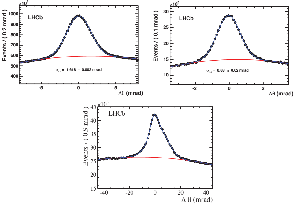
Fig. 37. \Delta\theta_C distributions for the RICH1 gas (top left), RICH2 gas (top right) and Aerogel (bottom). 82
