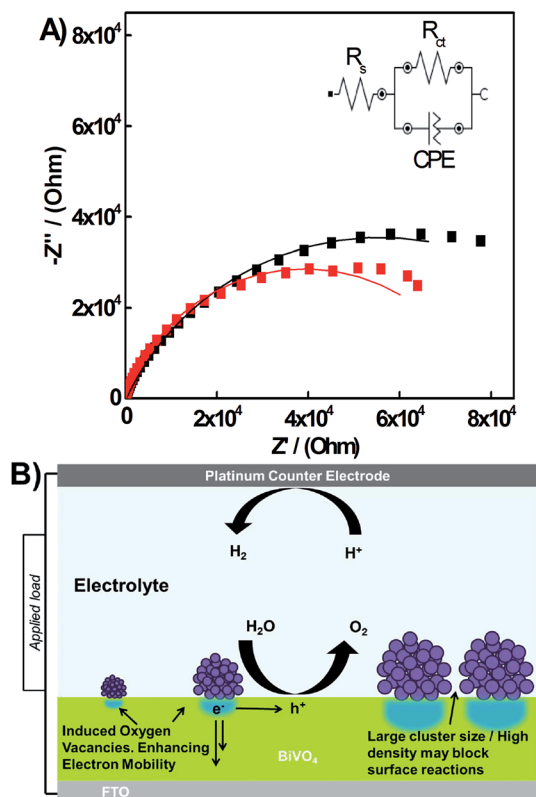
Fig. 7 (A) Nyquist plot for \text{BiVO}_4 photoelectrodes measured, under blue light illumination at 1.23 V vs. RHE, with (red) and without (black) \text{Ti}_{2000 \pm 54} clusters deposited at an average density of 3.5 \times 10^{10} clusters per \text{mm}^2 ; (B) schematic illustration outlining the photocurrent enhancement mechanism of different sized clusters on the surface of \text{BiVO}_4 .
