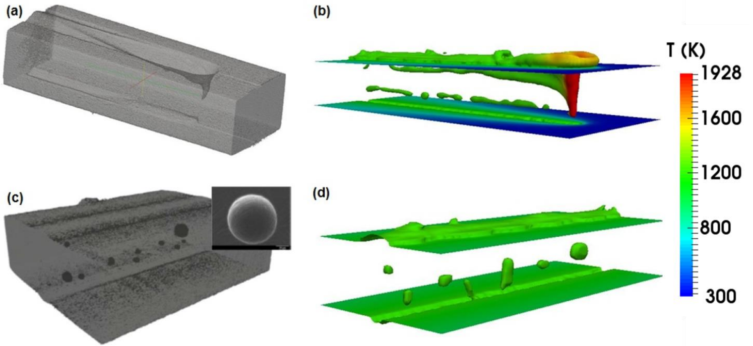
Figure 9: Comparison between (a) a partially collapsed keyhole surface using the reconstructed 3D X-ray tomography, after [14], and (b) keyhole modelling prediction of the liquid/vapour interface with 1mm thickness, 4000W and 100mm/s captured at the melting front, and between (c) pore distribution inside the weld bead reconstructed from X-ray tomography and (d) porosity prediction at the same condition as (b) but after solidification.
