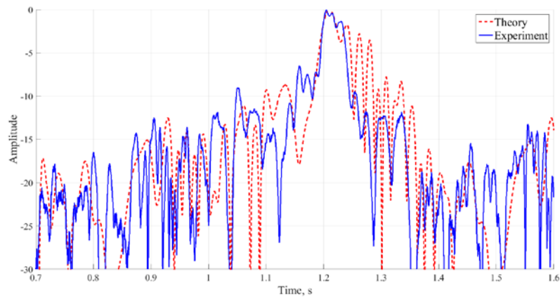
Fig. 18: Comparison between theoretical and experimental time-domain signatures.
