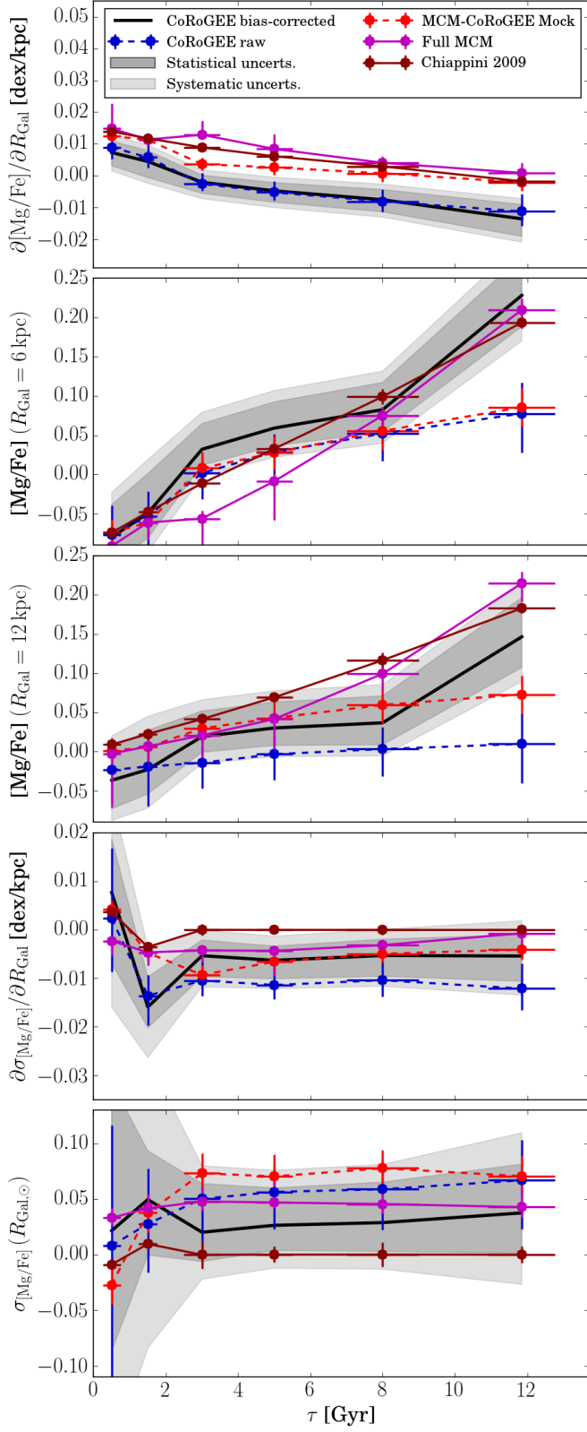
Fig. 8. Results of our four-parameter fits for the [\text{Mg}/\text{Fe}] vs. R_{\text{Gal}} distributions, in the same style as Fig. 3.
