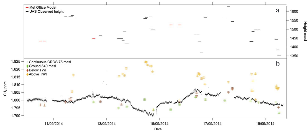
Figure 1. (a) The boundary layer heights per day calculated from either the temperature and humidity sensors on the UAS (black) or from the Met Office model (red). (b) Continuous CRDS \text{CH}_4 ground level (75 m asl) compared with bag samples taken during the September 2014 campaign, date markers denote 00 Coordinated Universal Time (UTC). The correlation between CRDS values and ground bag samples r^2 = 0.558 where critical r^2 = 0.247 at 0.05 significance. The bag samples have a negative bias of 2 ppb compared to the continuous CRDS values perhaps due to the sampling height difference. Using the difference between the median and the 95th percentile of the ground, below TWI, and above the TWI samples as a benchmark; ground level values give a difference of 3 ppb, below the TWI gives a difference of 7 ppb, and above the TWI mixing ratios gives a difference of 8 ppb. The difference of the median mixing ratios below and above the TWI is 16 ppb.
