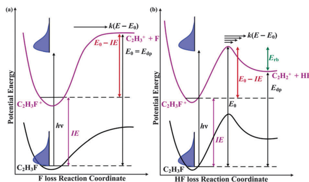
Fig. 1 Energy diagram for the dissociations of (a) \text{C}_2\text{H}_3\text{F}^+ into \text{C}_2\text{H}_3^+ + \text{F} without and (b) \text{C}_2\text{H}_3\text{F}^+ into \text{C}_2\text{H}_2^+ + \text{HF} with a reverse barrier. IE is the ionization energy, E_{\text{dp}} is the dissociative photoionization energy, E_{\text{rb}} is the height of the reverse barrier, E_0 is the 0 K appearance energy at which the products are first energetically accessible in the absence of tunnelling, and E_0 - IE is the height of the forward barrier. When there is no reverse barrier present, E_0 = E_{\text{dp}} .
